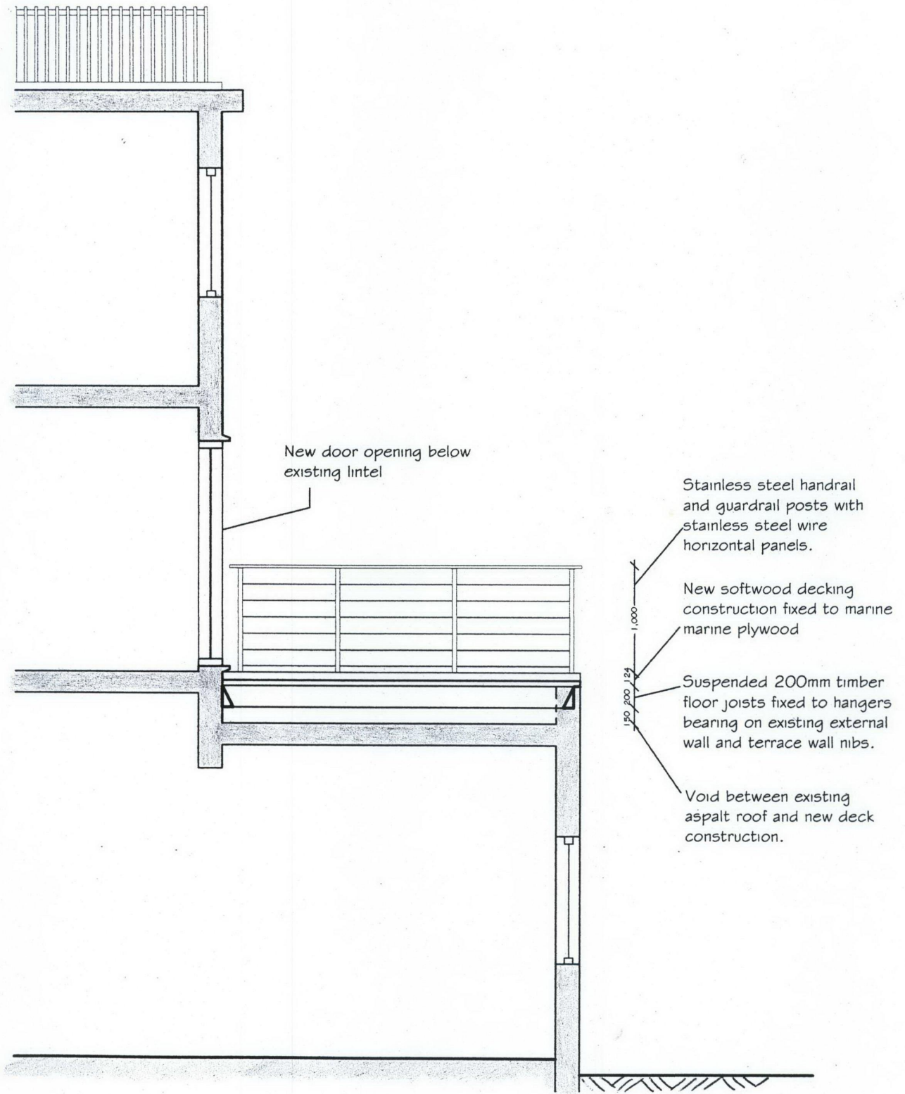
PROPOSED SECTION
