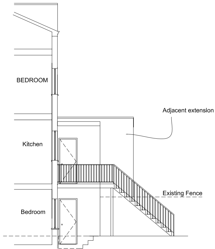
EXISTING EAST ELEVATION 1:100
