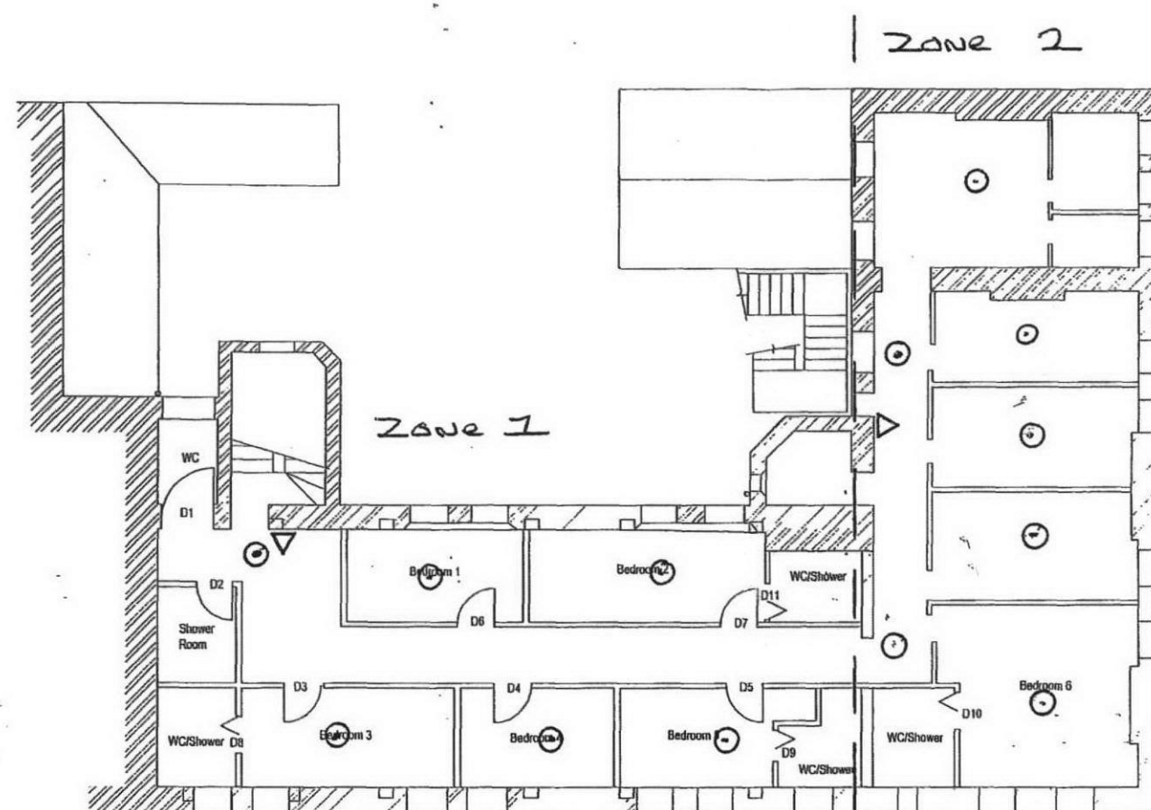
Proposed First Floor Layout 1:100 @ A3
