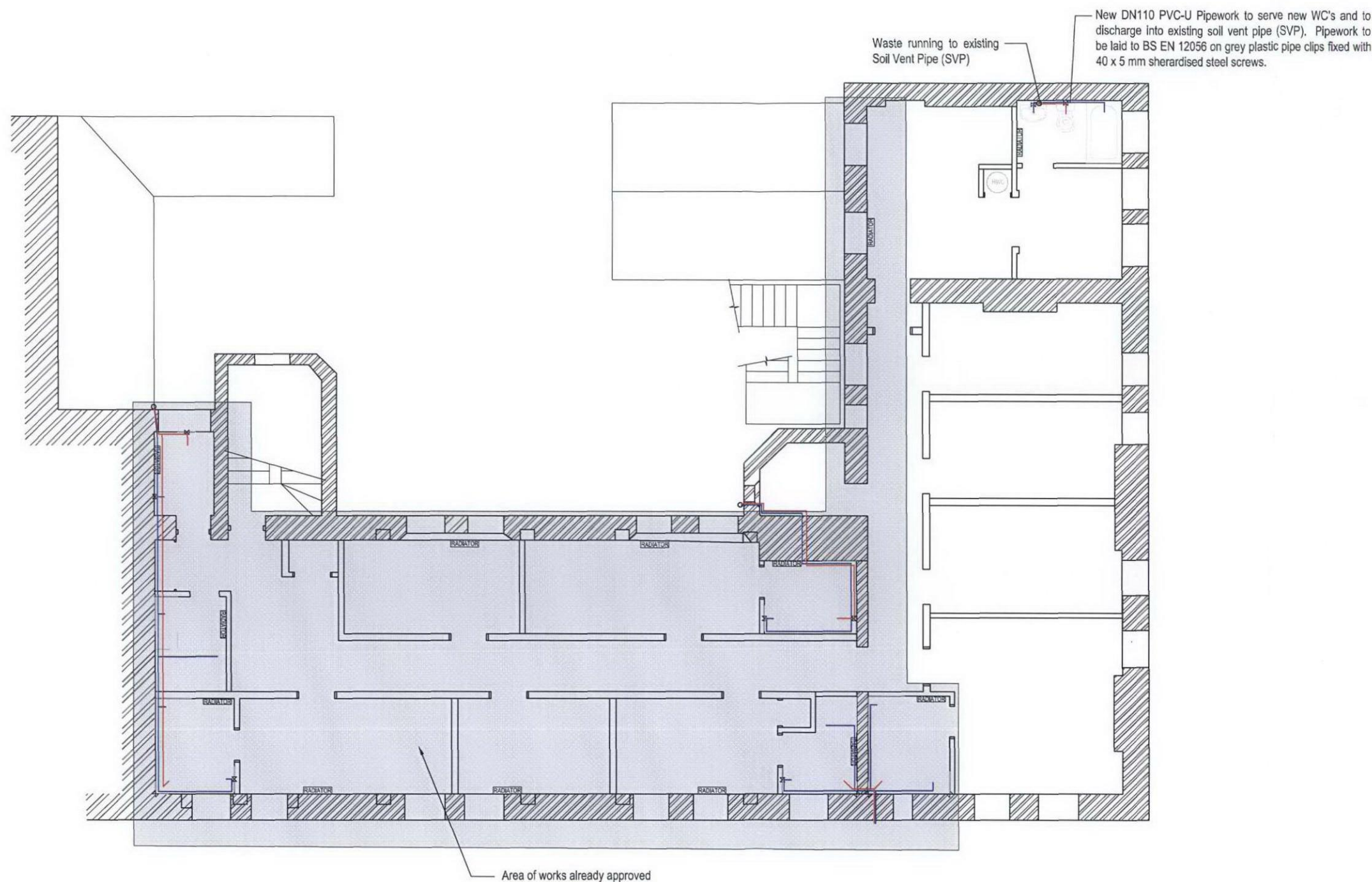
Proposed First Floor Layout 1:100 @ A3
