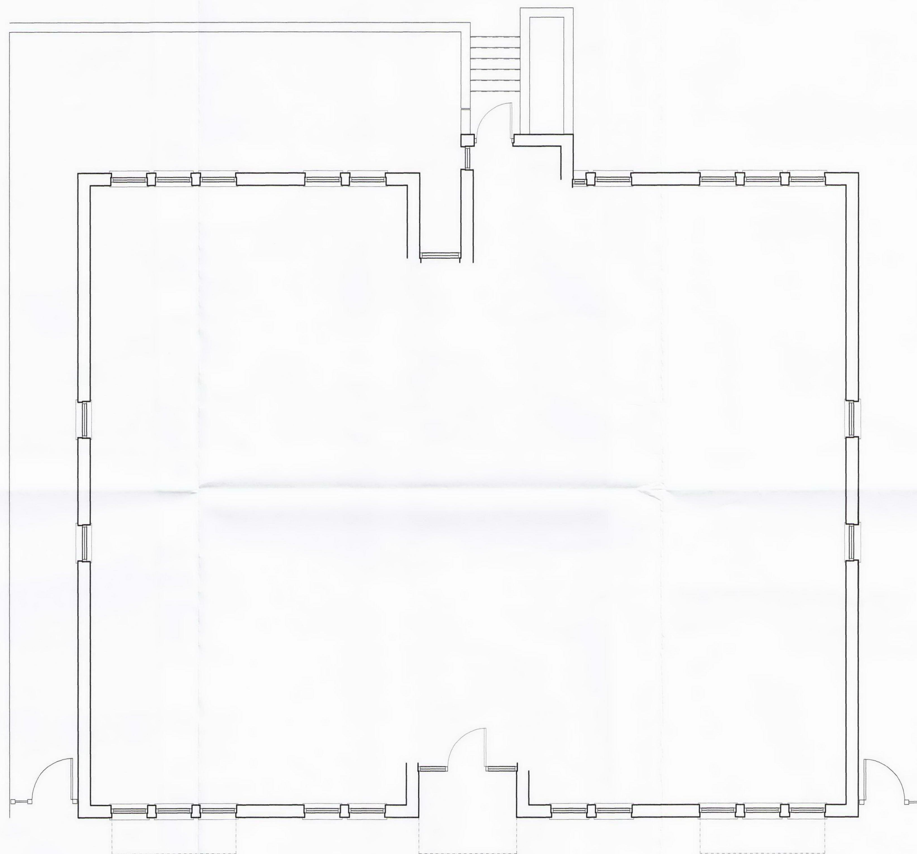
EXISTING INTERMEDIATE FLOOR PLAN SCALE 1:50
