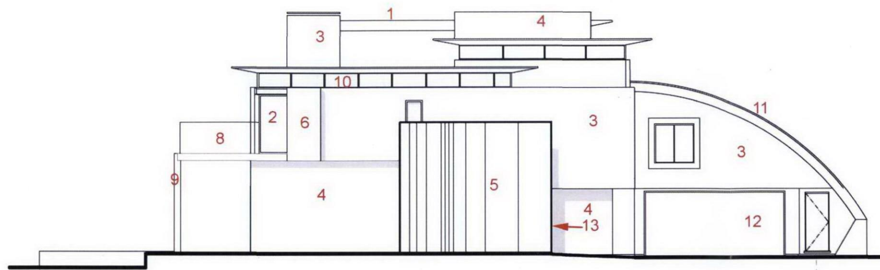
East Elevation
