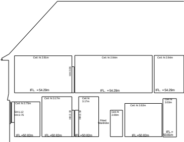
Section 'C' - 'C' Datum Level = 48.00 m
