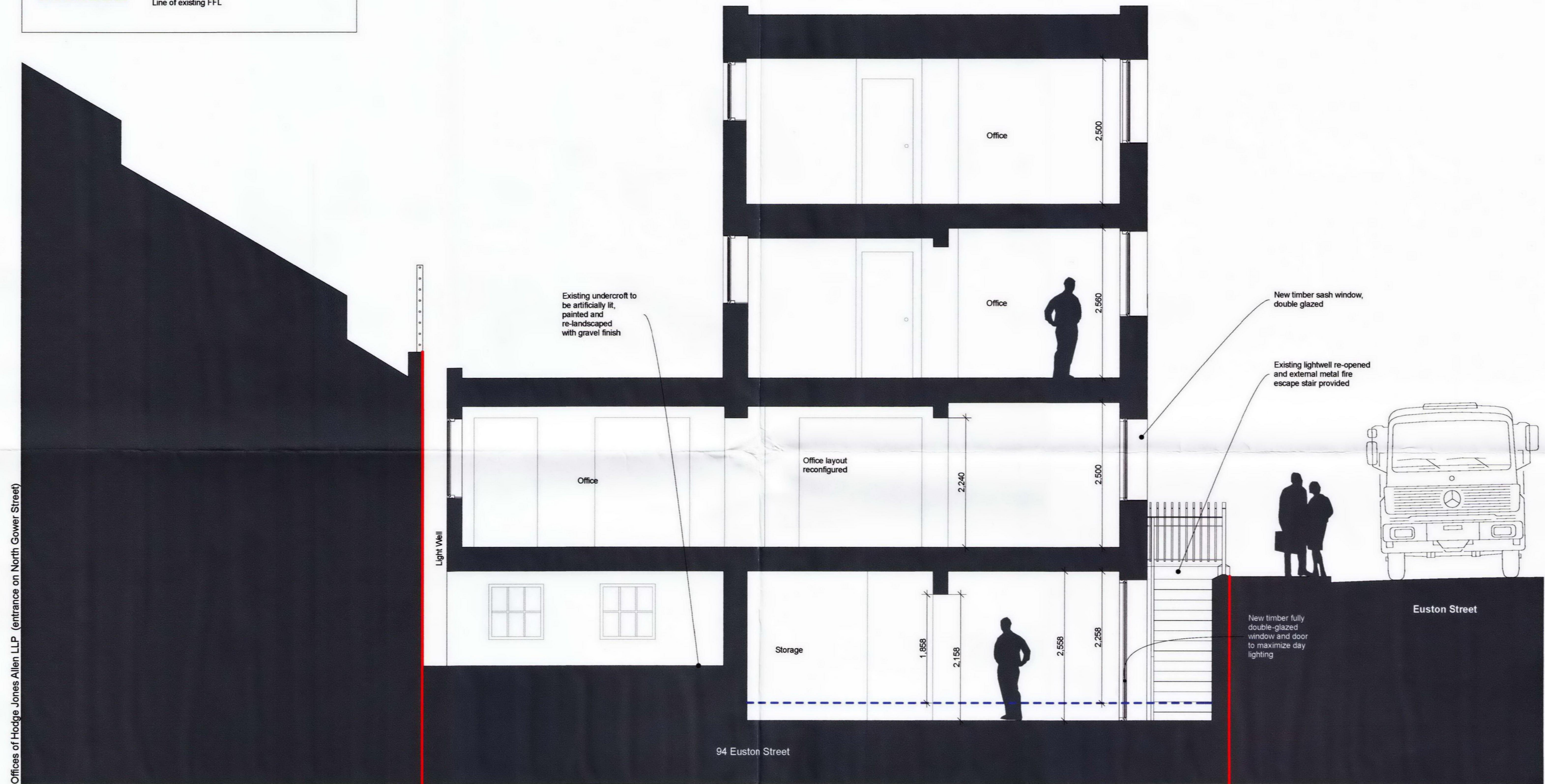
Section AA through 94 Euston Street
