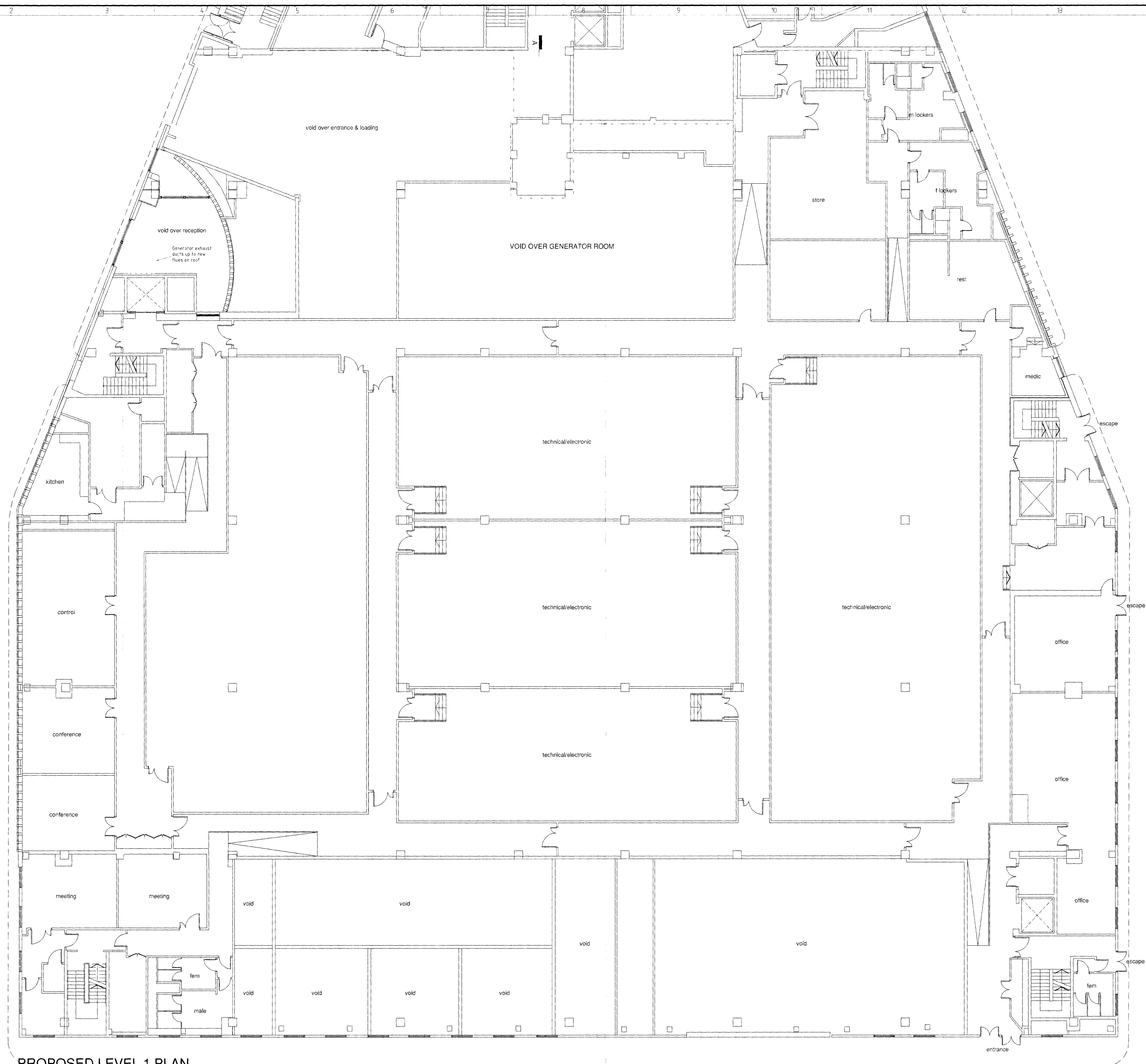
PROPOSED LEVEL 1 PLAN
