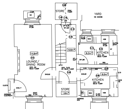
BASEMENT PLAN
