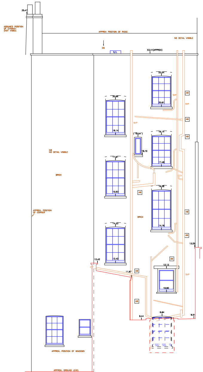
REAR ELEVATION
