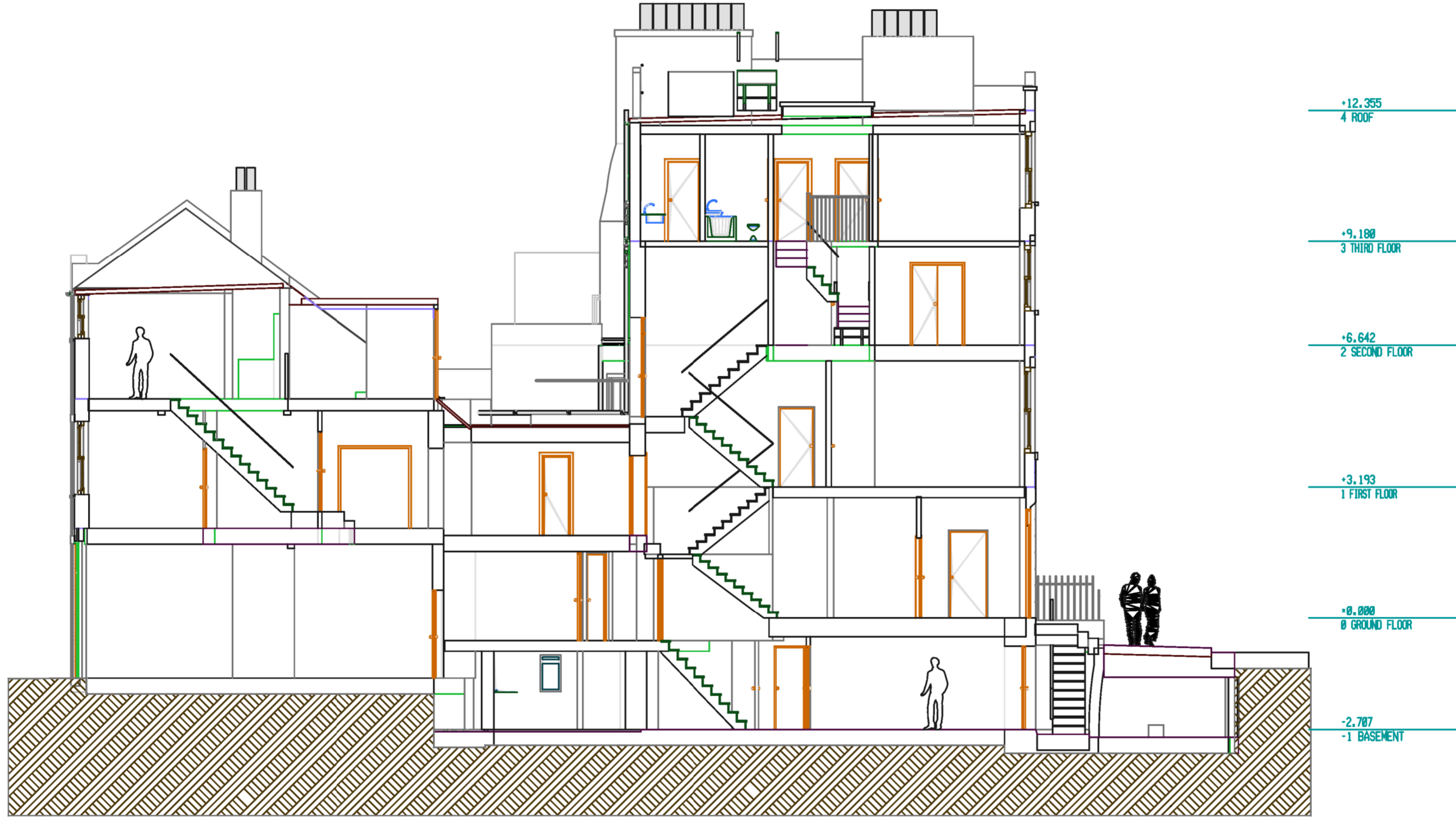
LONG SECTION A-A THROUGH MAIN HOUSE & MEWS
