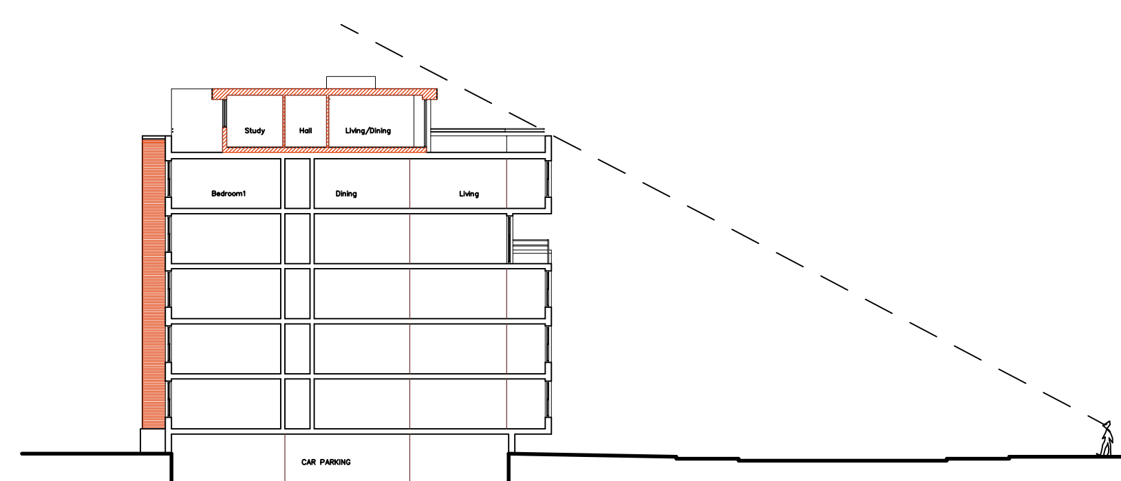
CROSS SECTION SHOWING PROPOSED PENTHOUSE APARTMENT OVER FLATS 26-45
