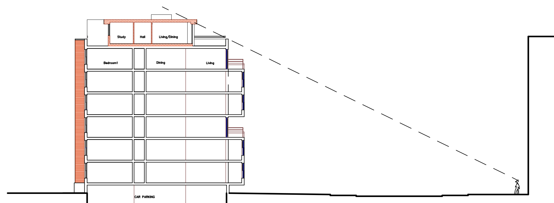
CROSS SECTION SHOWING PROPOSED PENTHOUSE APARTMENT OVER FLATS 46-65
