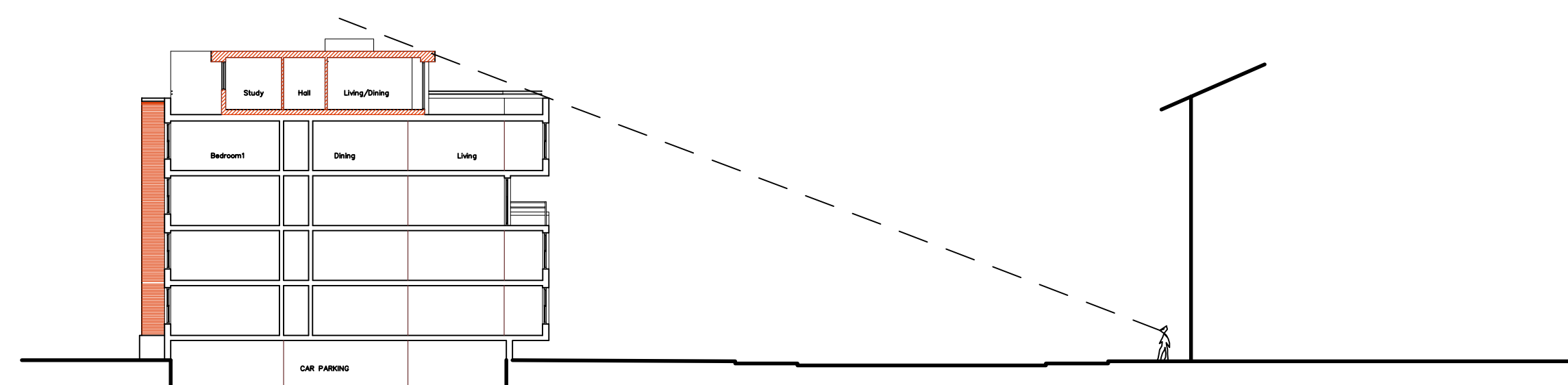
CROSS SECTION SHOWING PROPOSED PENTHOUSE APARTMENT OVER FLATS 90-105
