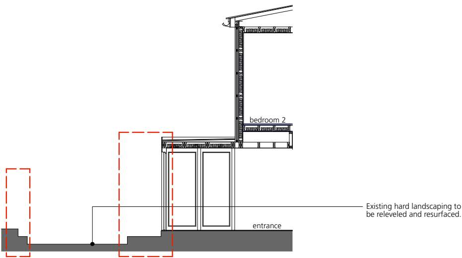
A Existing Section A-A PL_04
