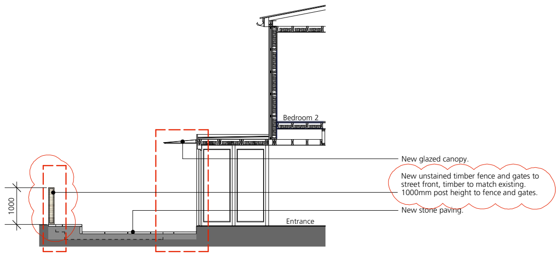
B Proposed Section B-B PL_04
