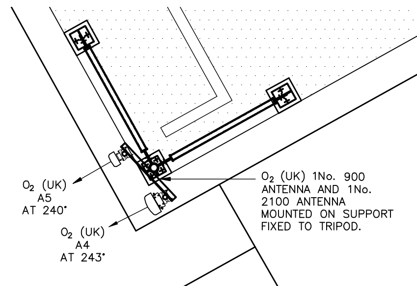
PROPOSED ANTENNA PLAN (CELL 2)
