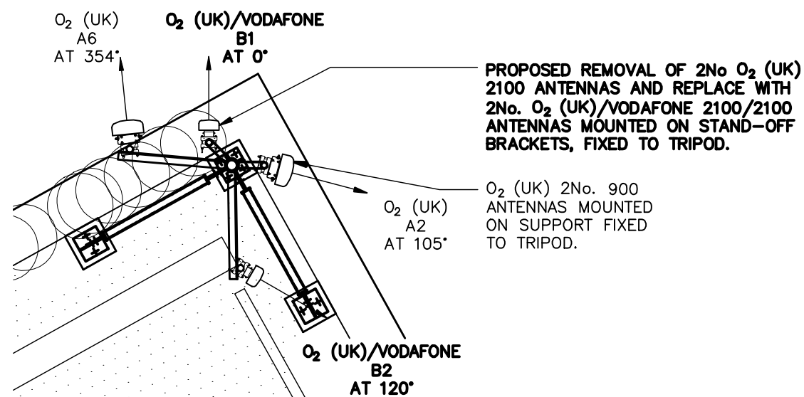
PROPOSED ANTENNA PLAN (CELLS 1 & 3)
