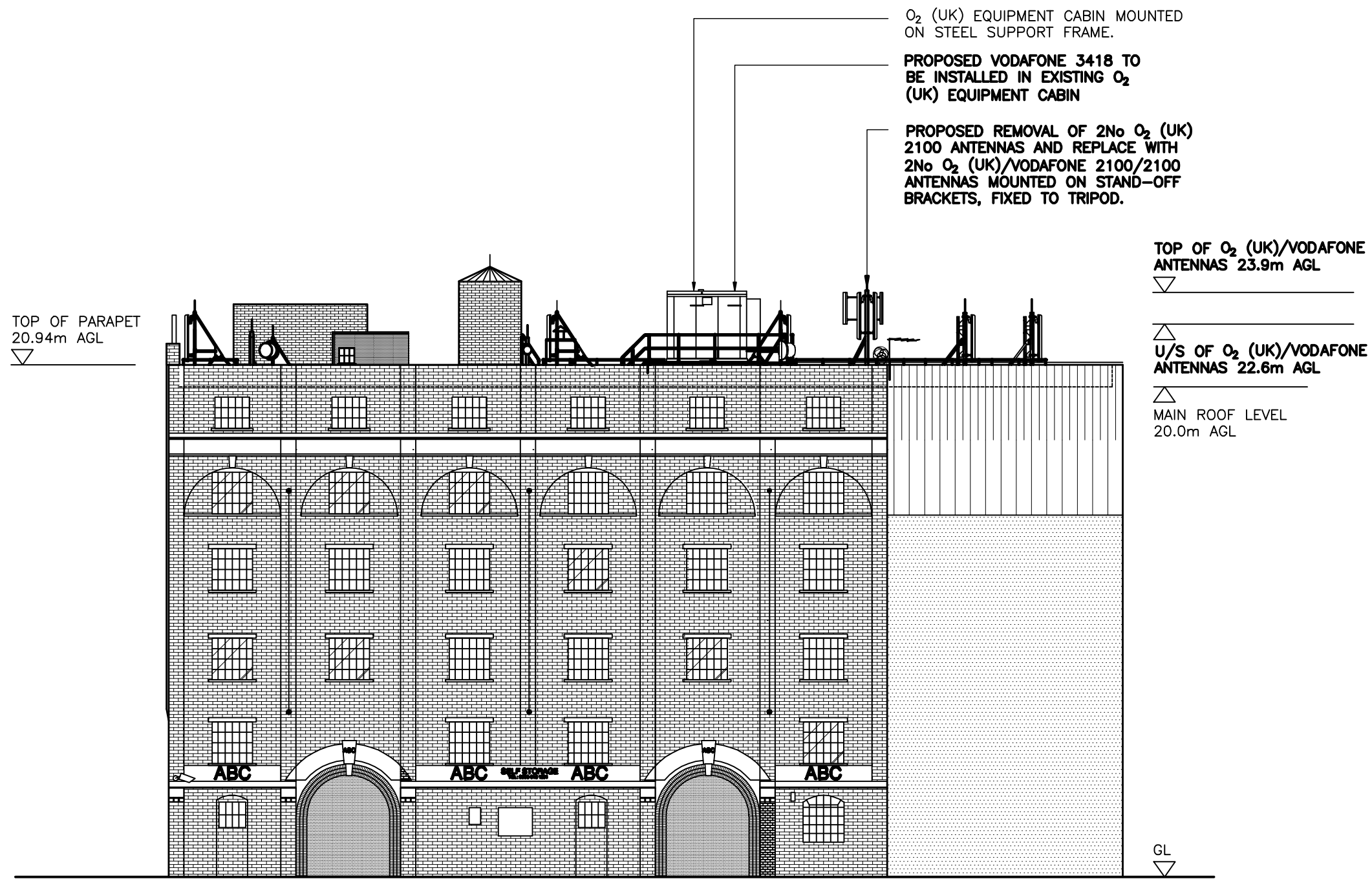
ELEVATION 'A' SCALE 1:200
