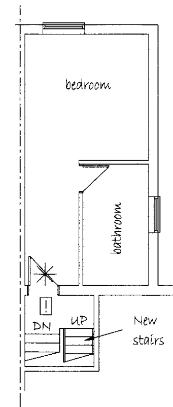
PROPOSED UPPER MEZZANINE LEVEL
