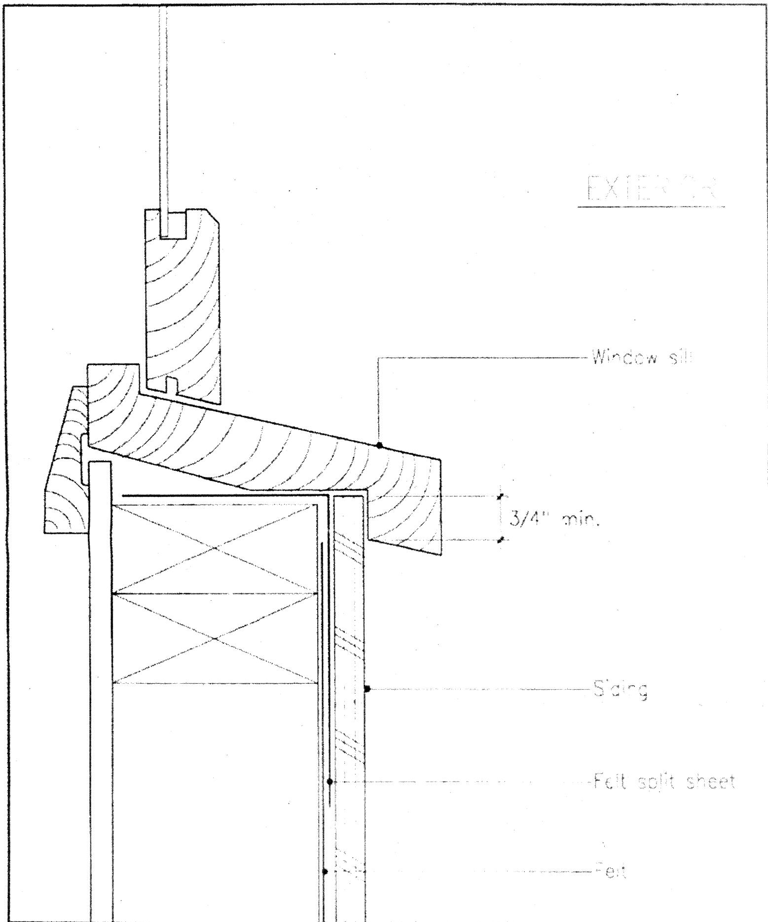
WOOD WINDOW DETAIL SILL DETAIL IN PLYWOOD SIDING
