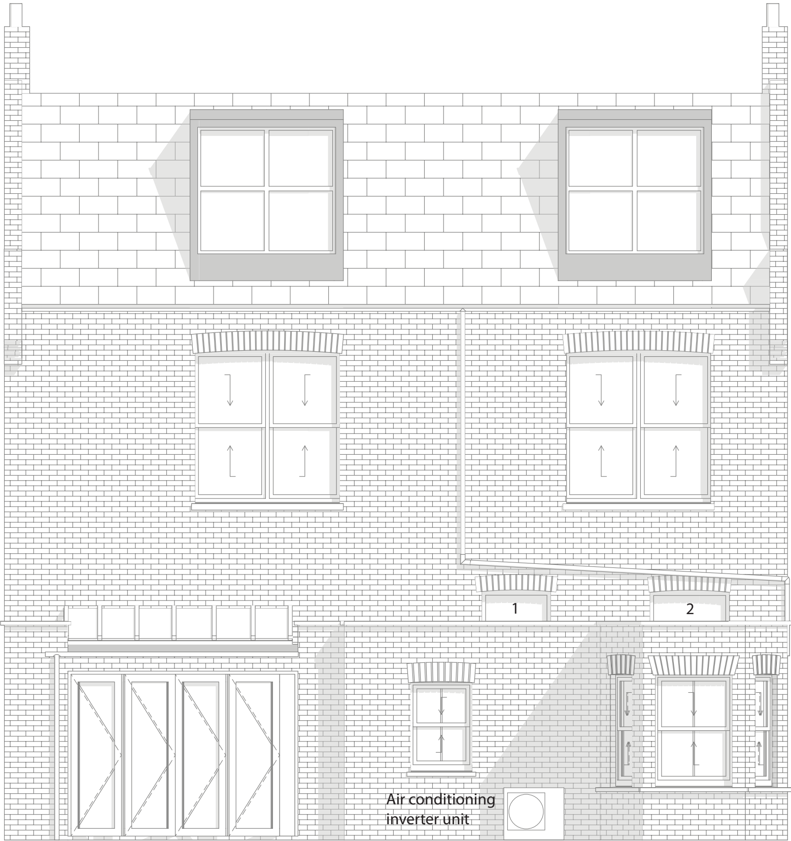
REAR ELEVATION POST DEVELOPMENT
