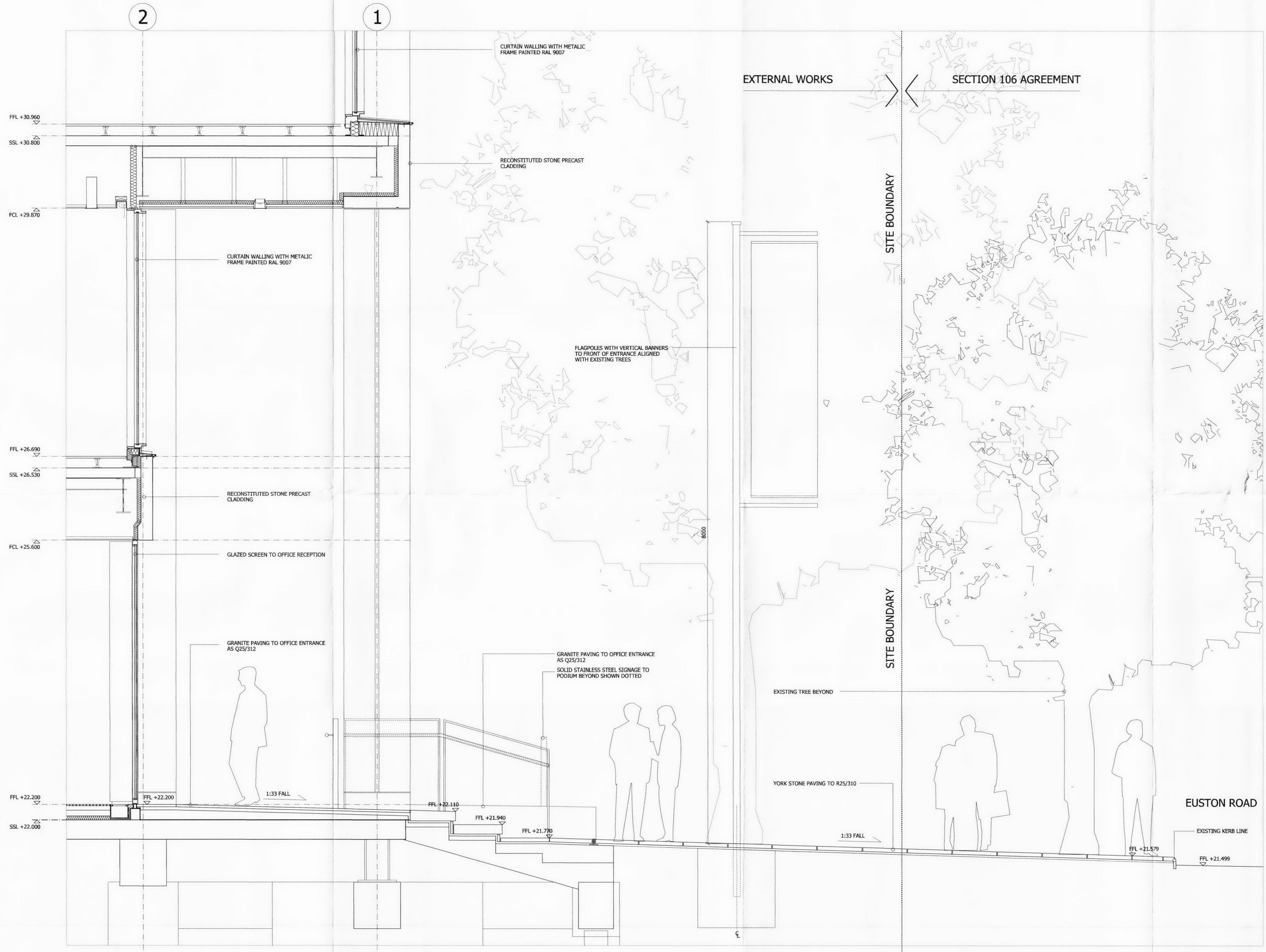
01 SECTION AA - OFFICE ENTRANCE 05070_Ext_Sect_Block A1 Entry Glazing_01.dgn
