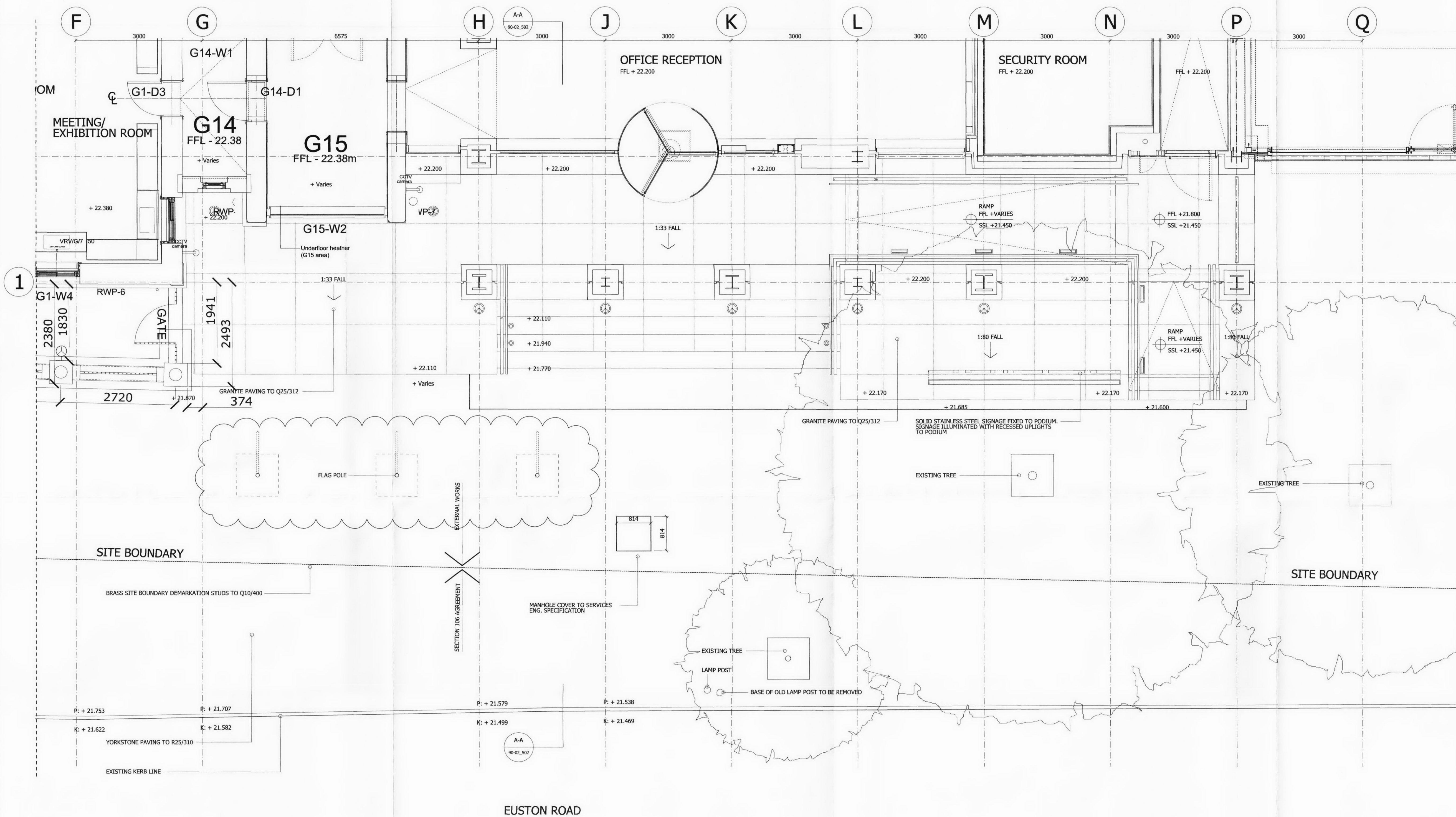
02 PLAN - RECEPTION ENTRANCE 05070_GA_Plan_GRO_01.dgn
