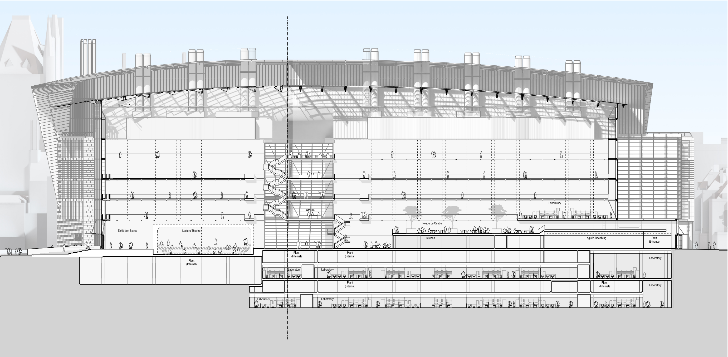
Fig 7-14. East-west section through central atrium
