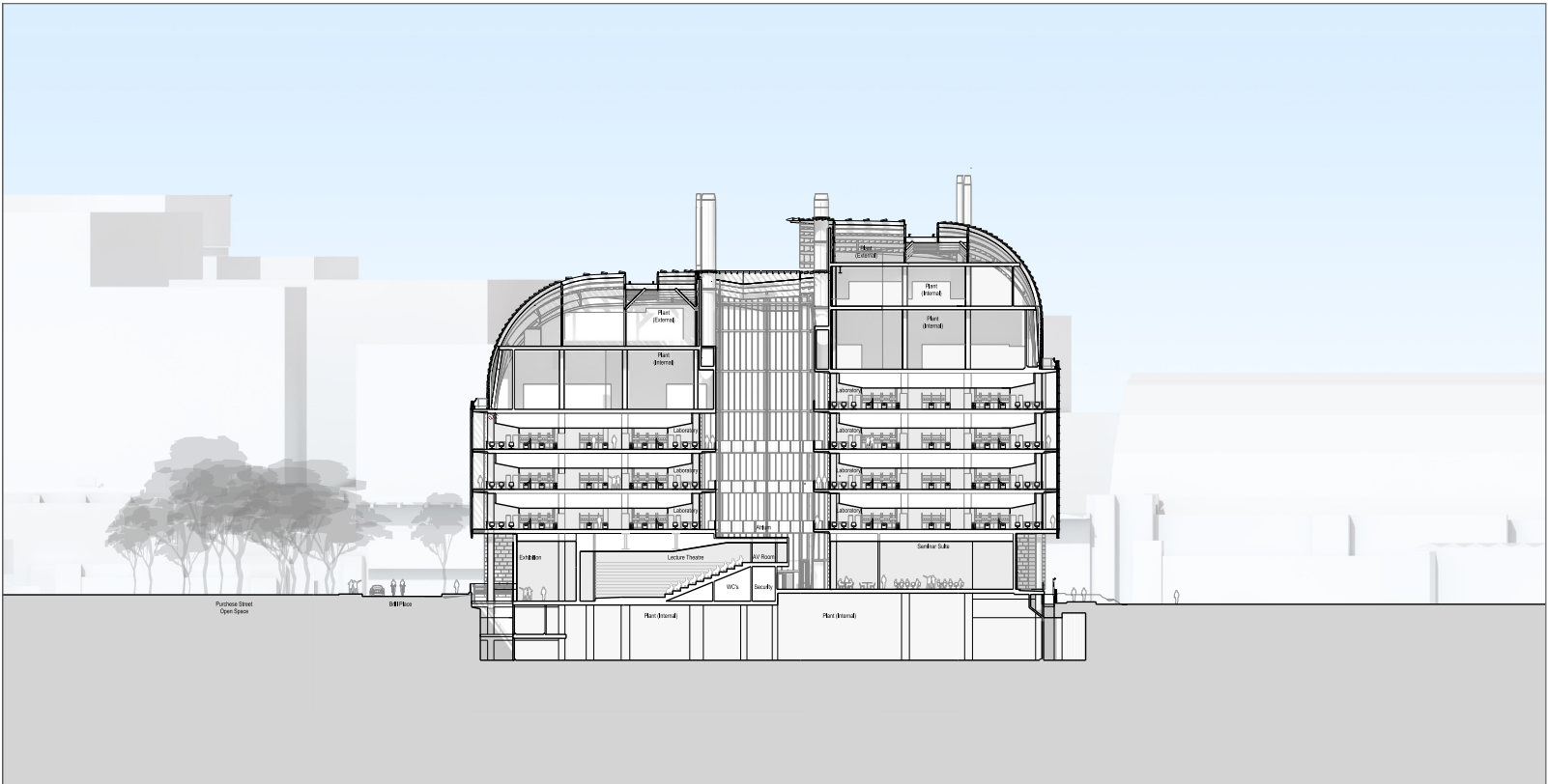
Fig 7-8. North-south section through laboratory wings
