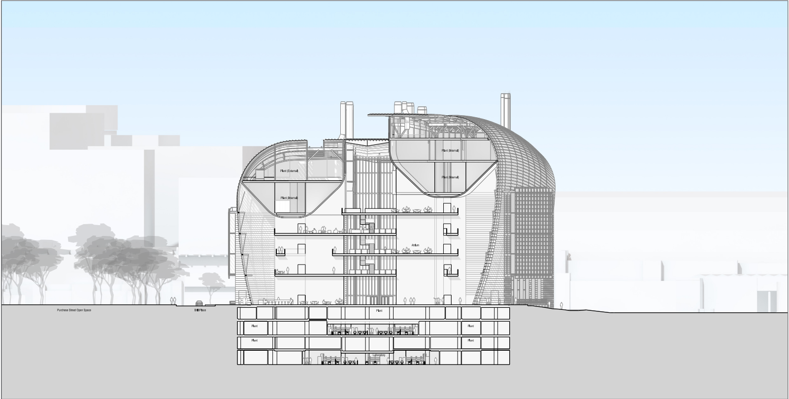
Fig 7-7. North-south section through cross atrium
