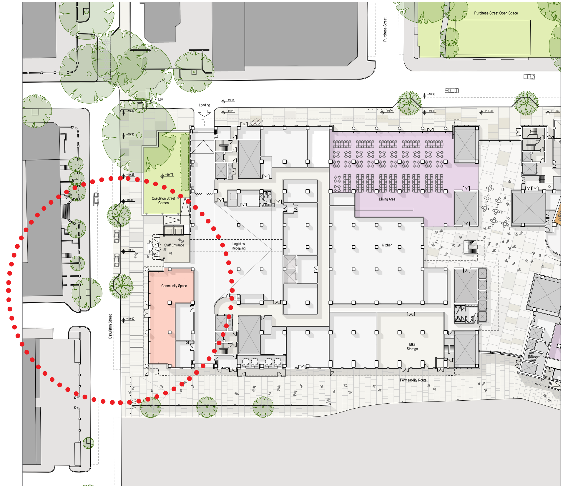
Fig 6-16. Public realm plan west; boundary trees are subject to approval of LBC as highways authority and effected utility companies
