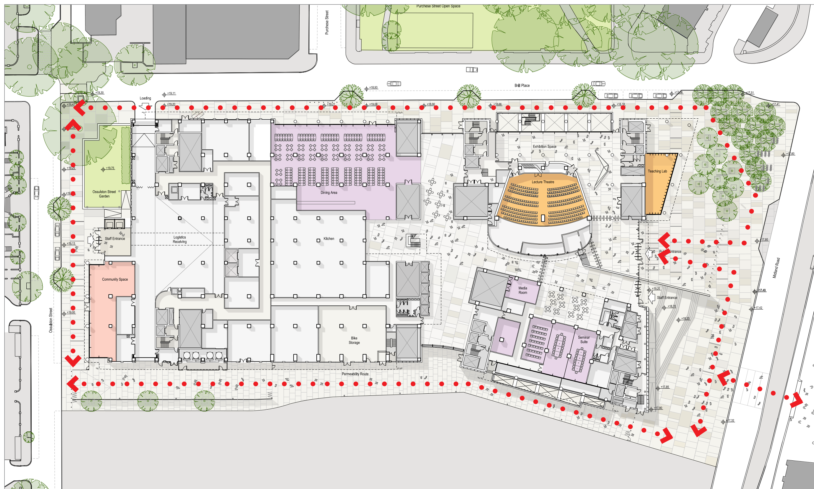
Fig 6-4. Public realm plan; boundary trees are subject to approval of LBC as highways authority and affected utility companies
