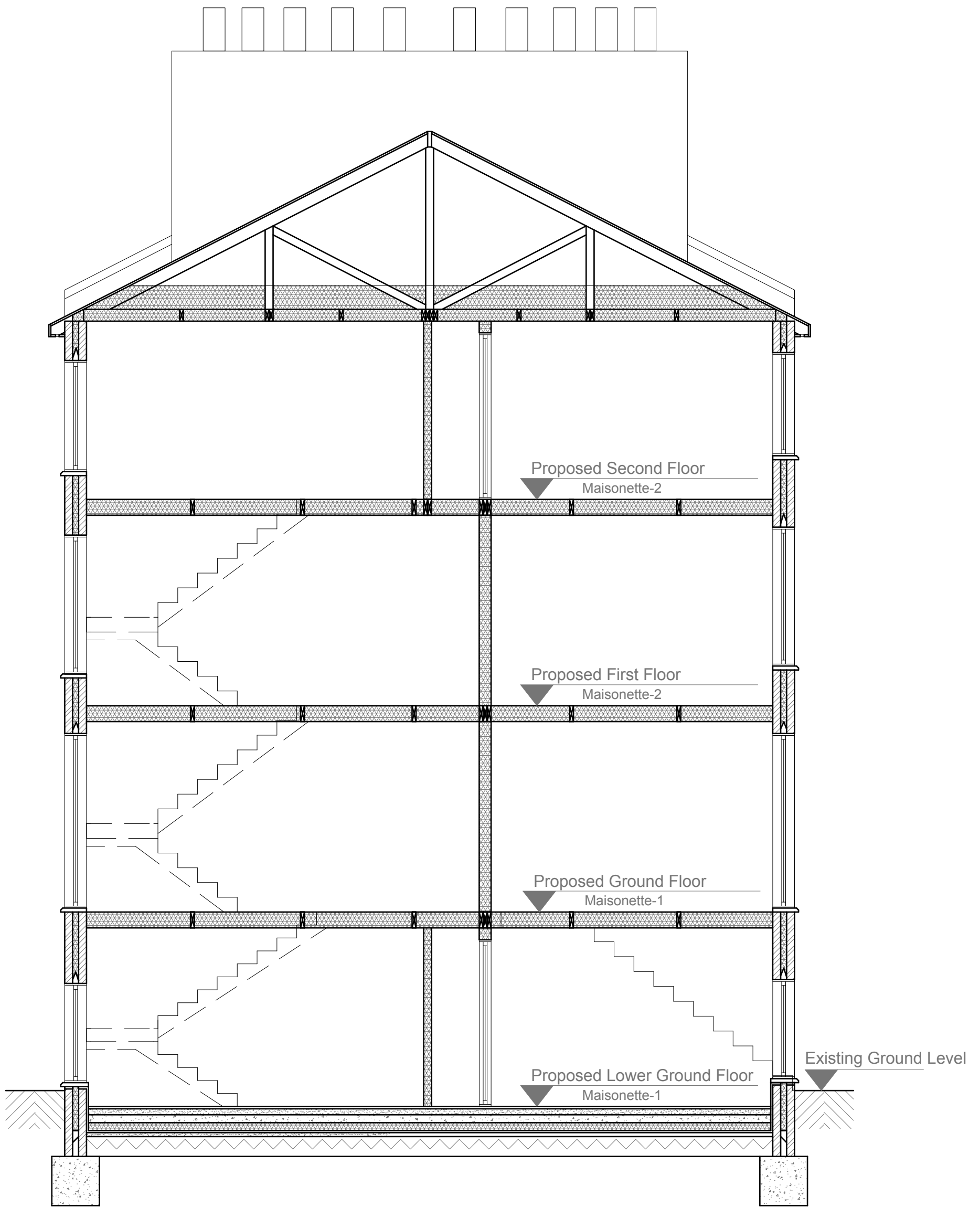
Proposed Section Scale 1:50
