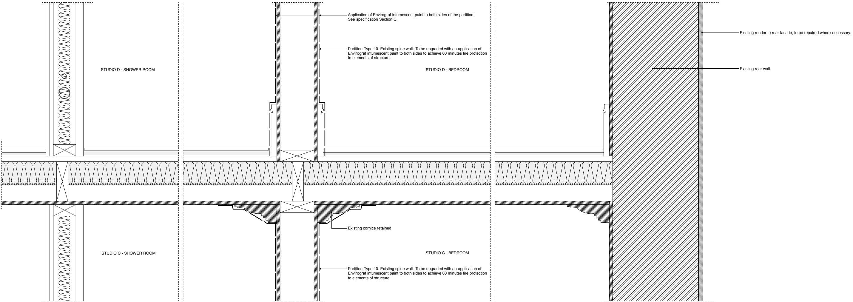
145.506.A - DETAIL SECTION THROUGH PROPOSED SECOND FLOOR CONSTRUCTION
