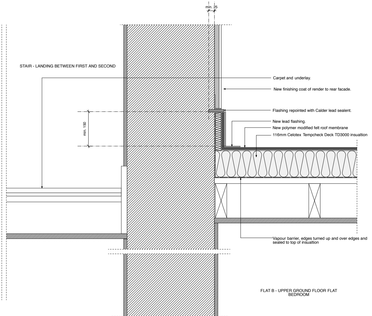
145.506.B - DETAIL SECTION THROUGH REAR ADDITION ROOF CONSTRUCTION
