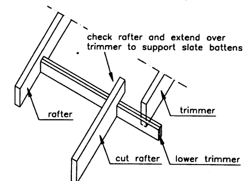
RAFTER / TRIMMER LAYOUT
