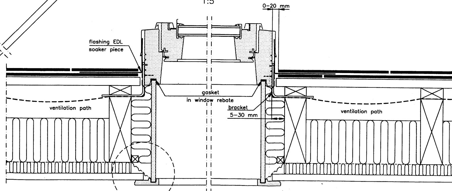
SECTION B-B 1:5
