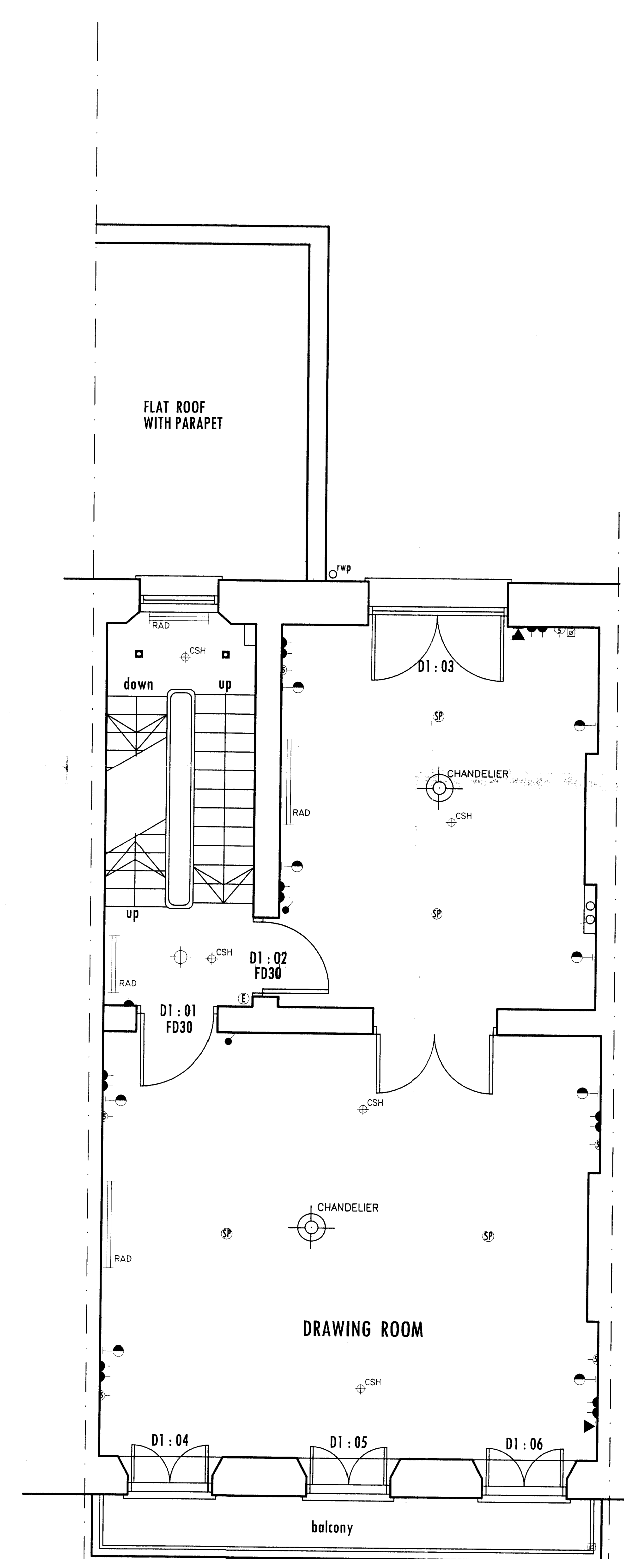
FIRST FLOOR PLAN - ELECTRICAL LAYOUT
