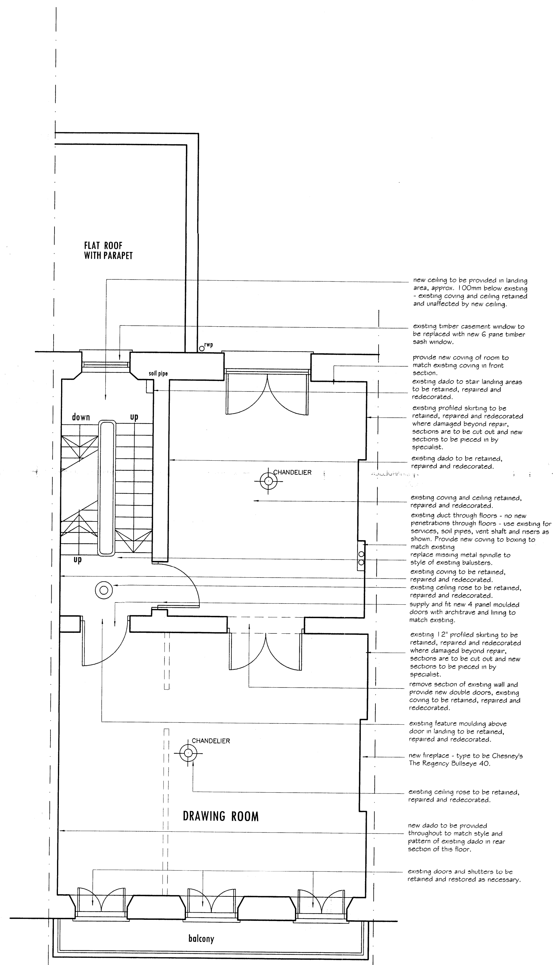
FIRST FLOOR PLAN AS PROPOSED
