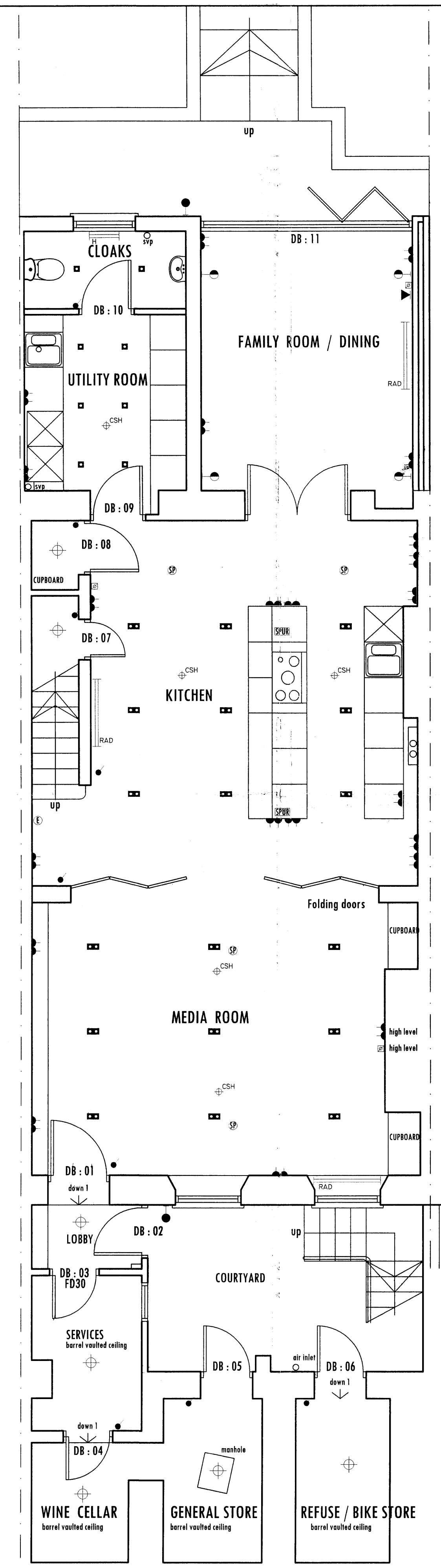
BASEMENT FLOOR PLAN ELECTRICAL LAYOUT
