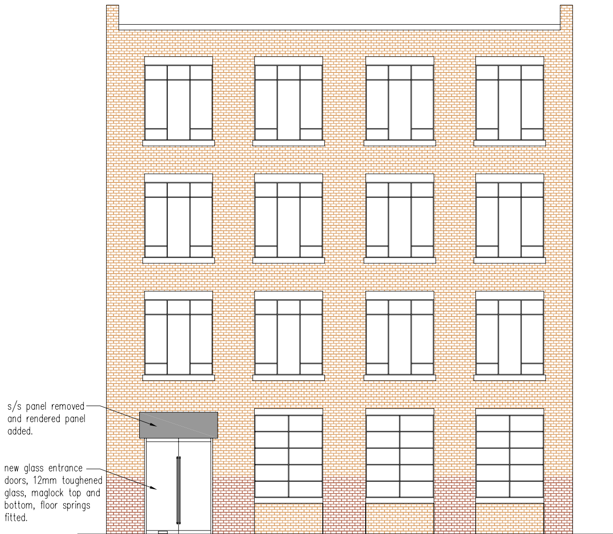
Proposed Elevation
