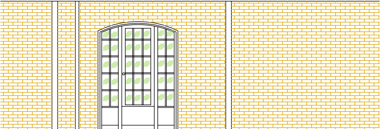
PROPOSED ELEVATION
