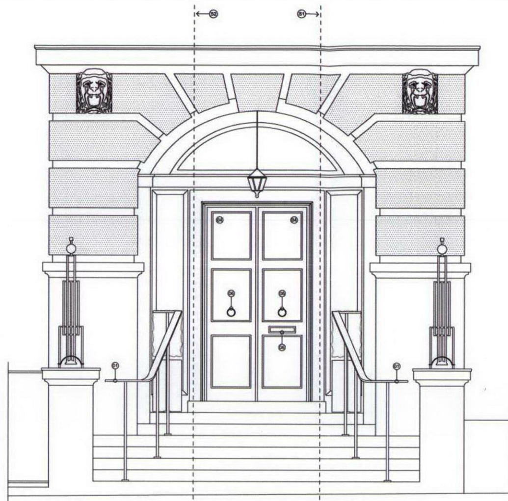
Proposed Elevation E1 Scale: 1:20 @ A1
