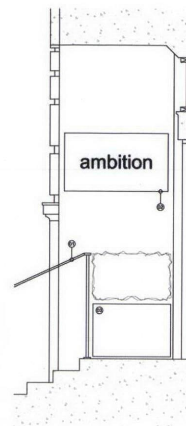
Proposed Section S2 Scale: 1:20 @ A1
