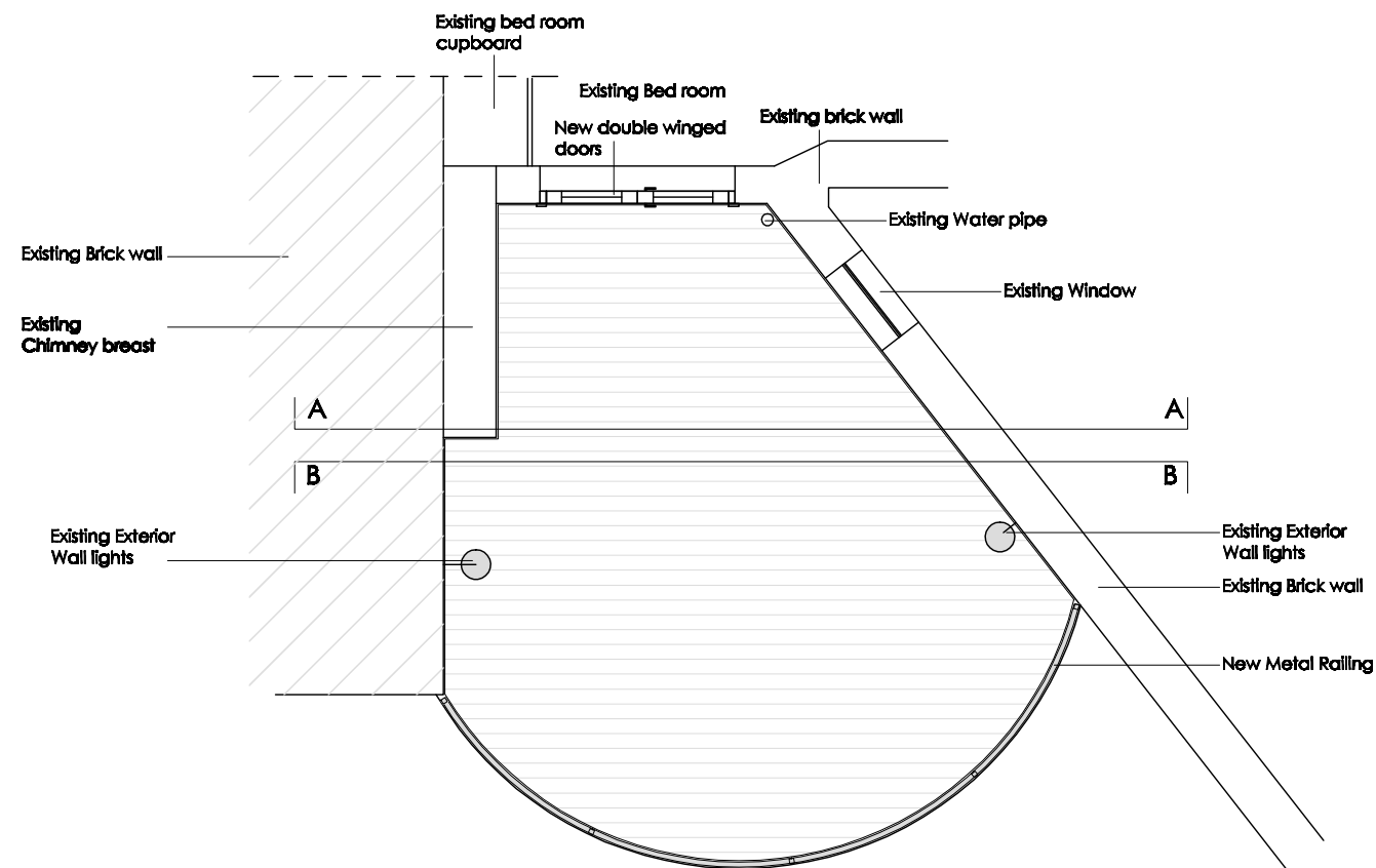
PLAN NEW TERRACE AND DOOR
