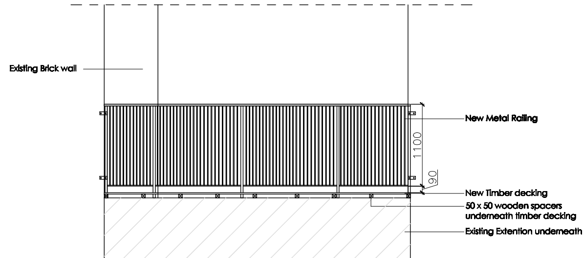
ELEVATION B-B NEW TERRACE AND DOOR
