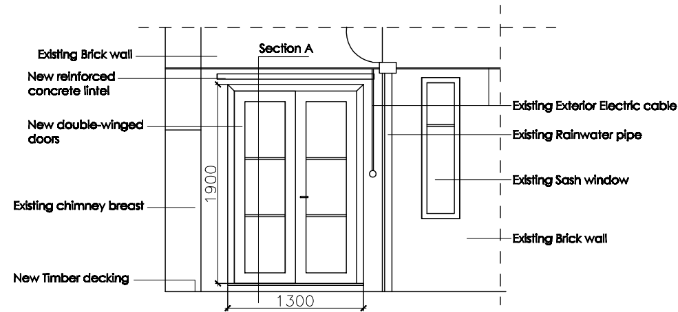
ELEVATION A-A NEW TERRACE AND DOOR
