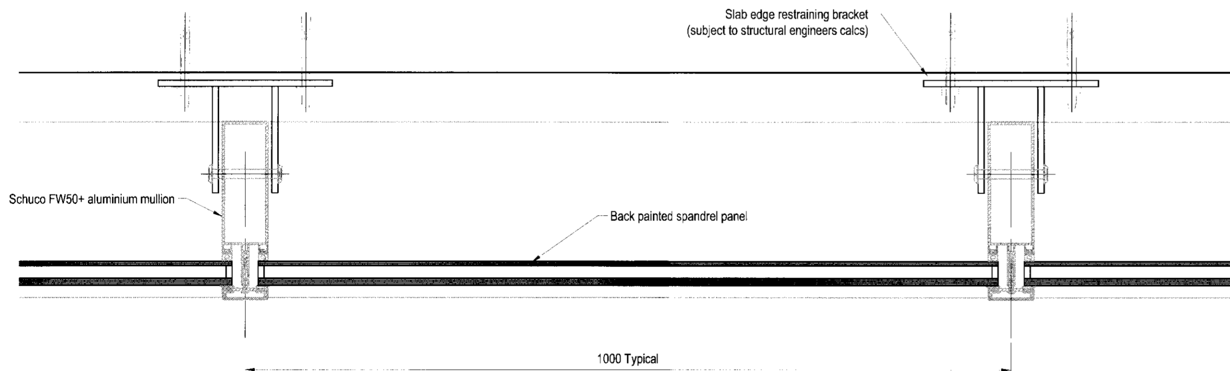
05 Typical horizontal section thro' facade at spandrel panel 1:20
