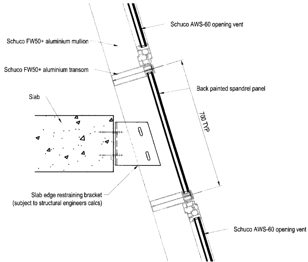
01 Typical vertical section thro' facade at slab edge (restraining bracket) 1:20
