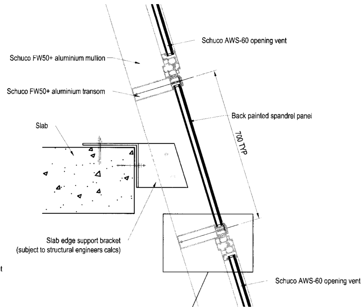
04 Enlarged detail 1:5
