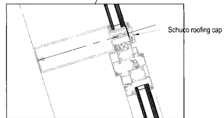
04 Enlarged detail 1:5
