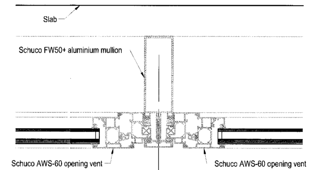
03 Typical horizontal section thro' mullion at vents 1:20
