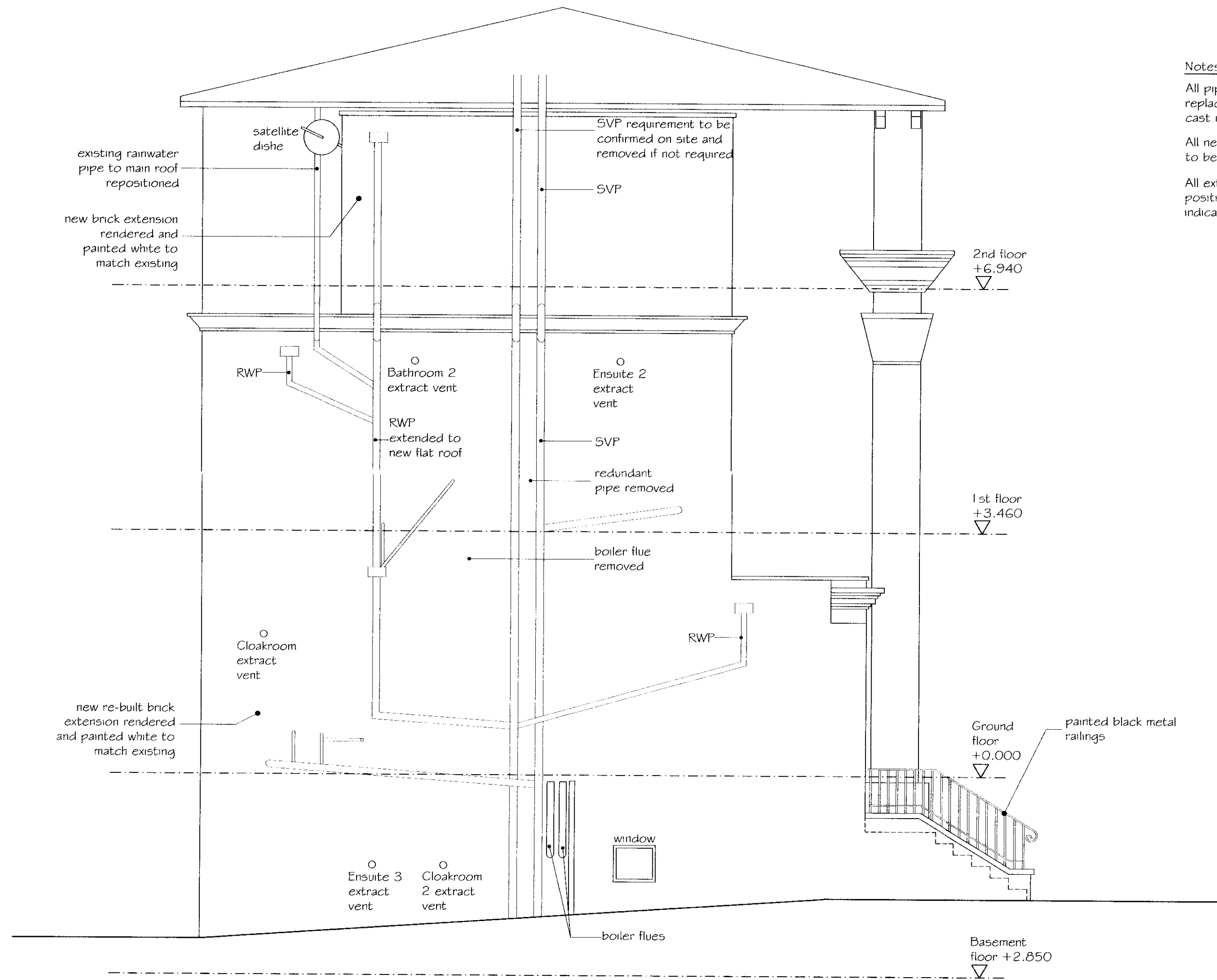
Proposed Side Elevation C - Scale 1:50
