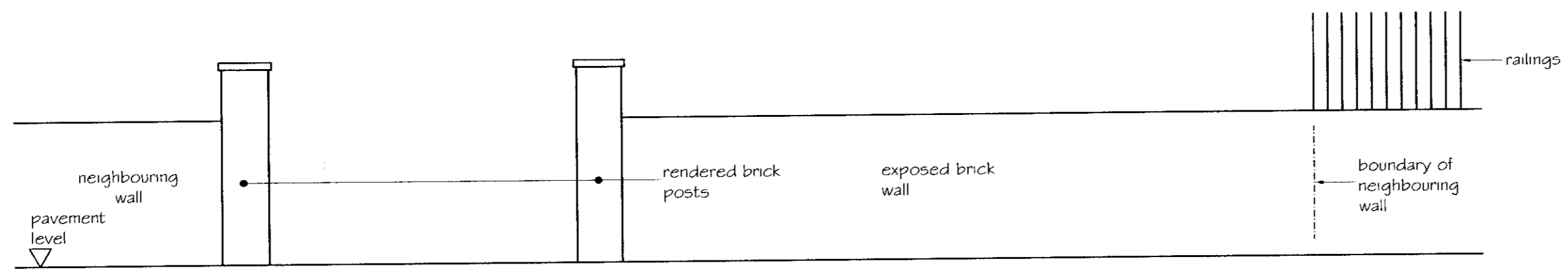
Existing Front Wall Elevation - Scale 1:50
