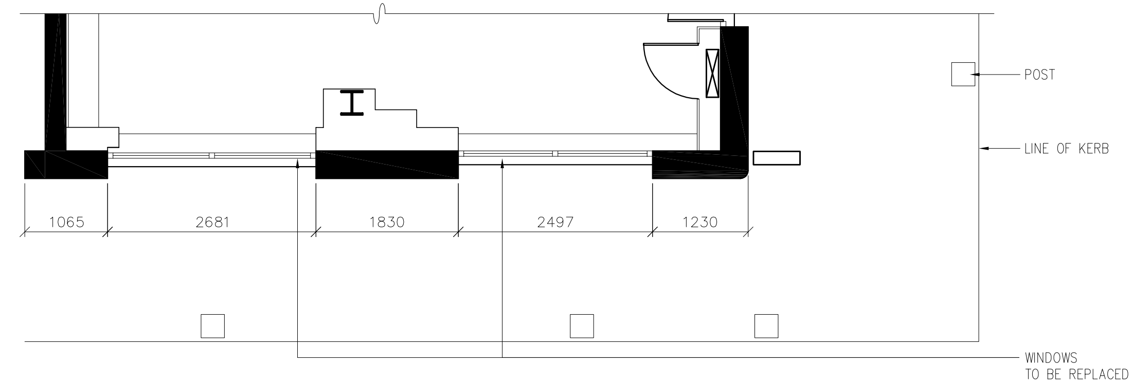
EXISTING PARTIAL PLAN VIEW
