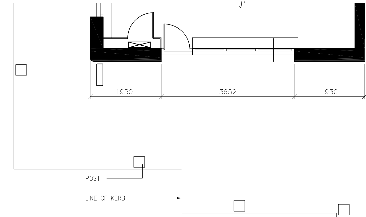
EXISTING PARTIAL PLAN VIEW
