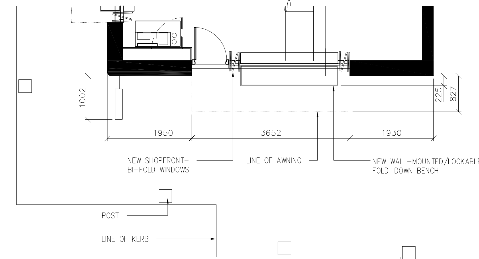
PROPOSED PARTIAL PLAN VIEW
