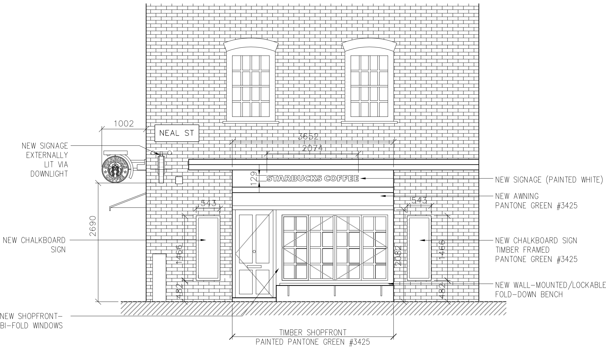
2 PROPOSED FRONT ELEVATION
