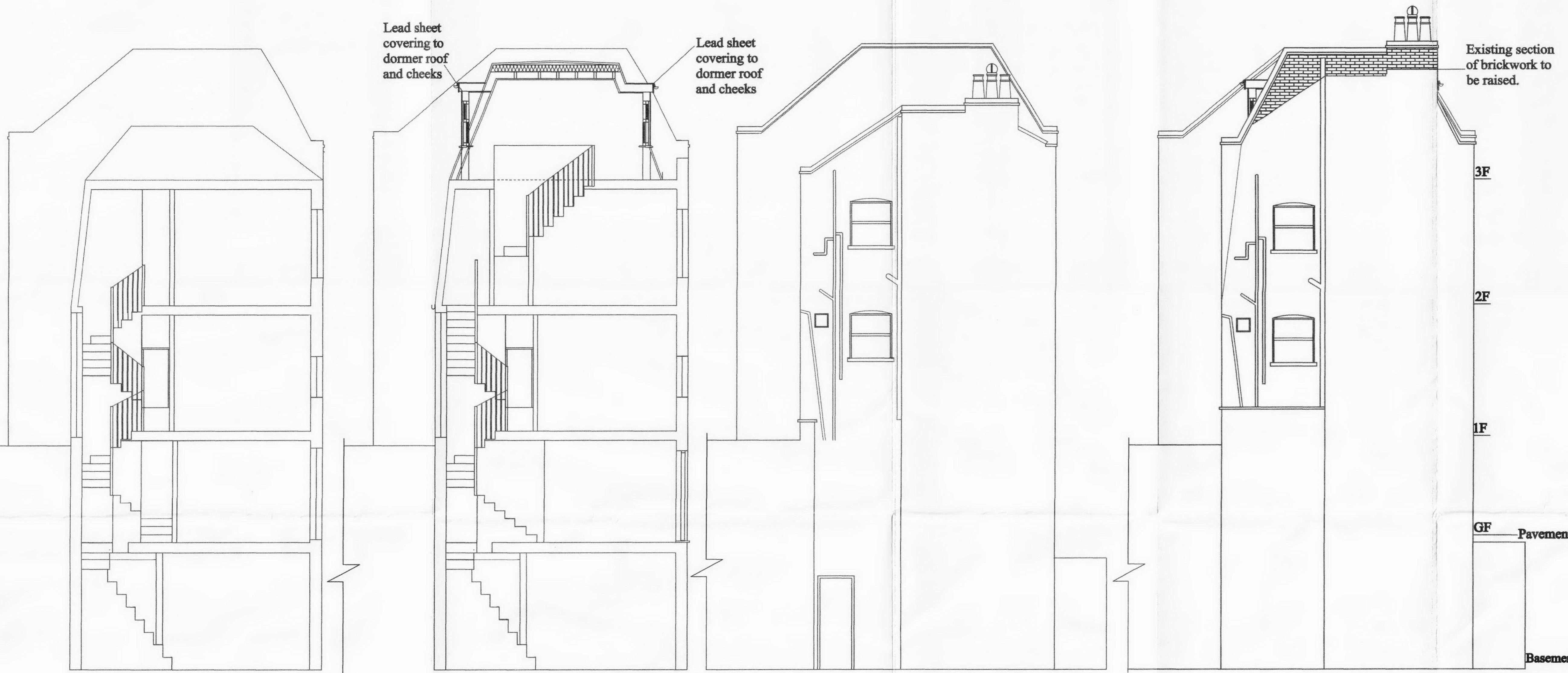
EXISTING SECTION A-A SCALE 1:50
