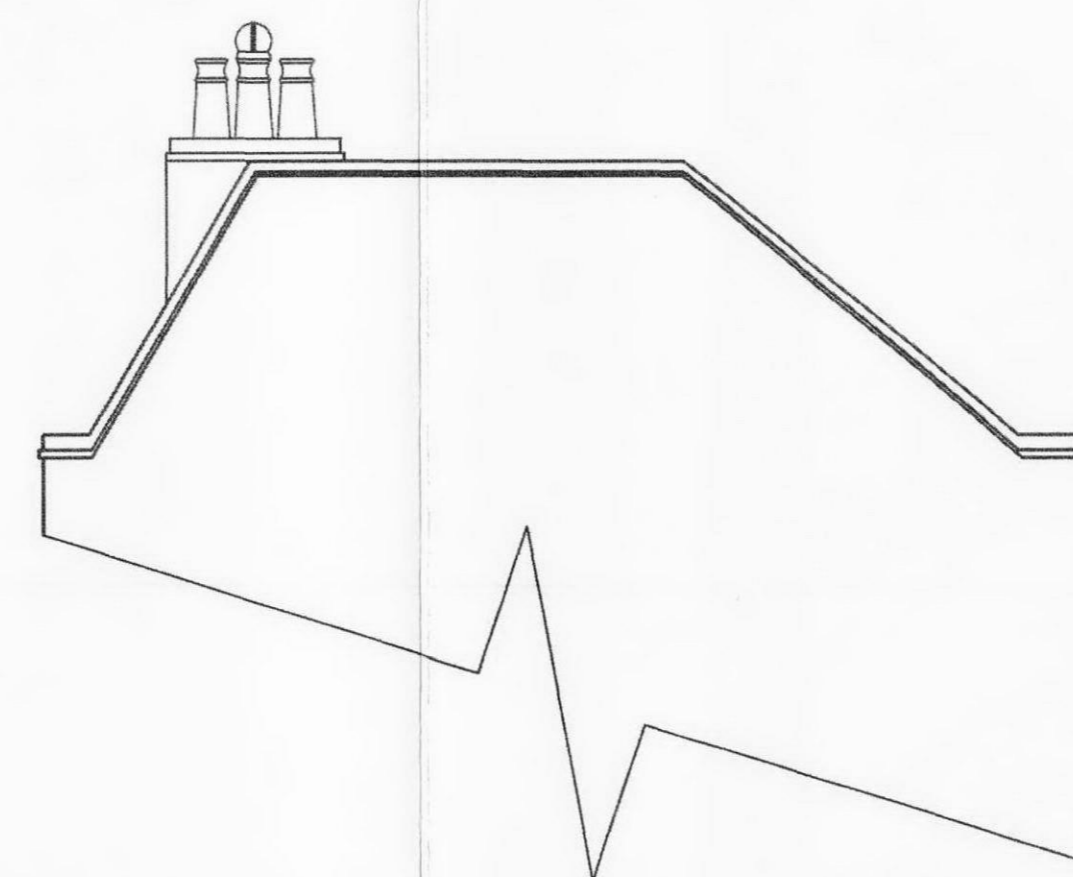
EXISTING RIGHT HAND SIDE ELEVATION SCALE 1:50
