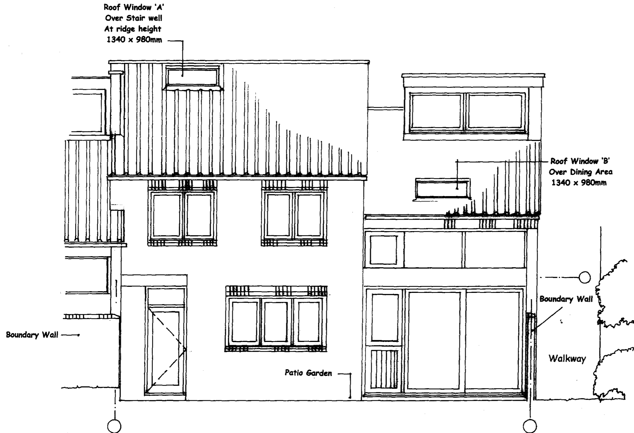
EXISTING & PROPOSED ELEVATION
