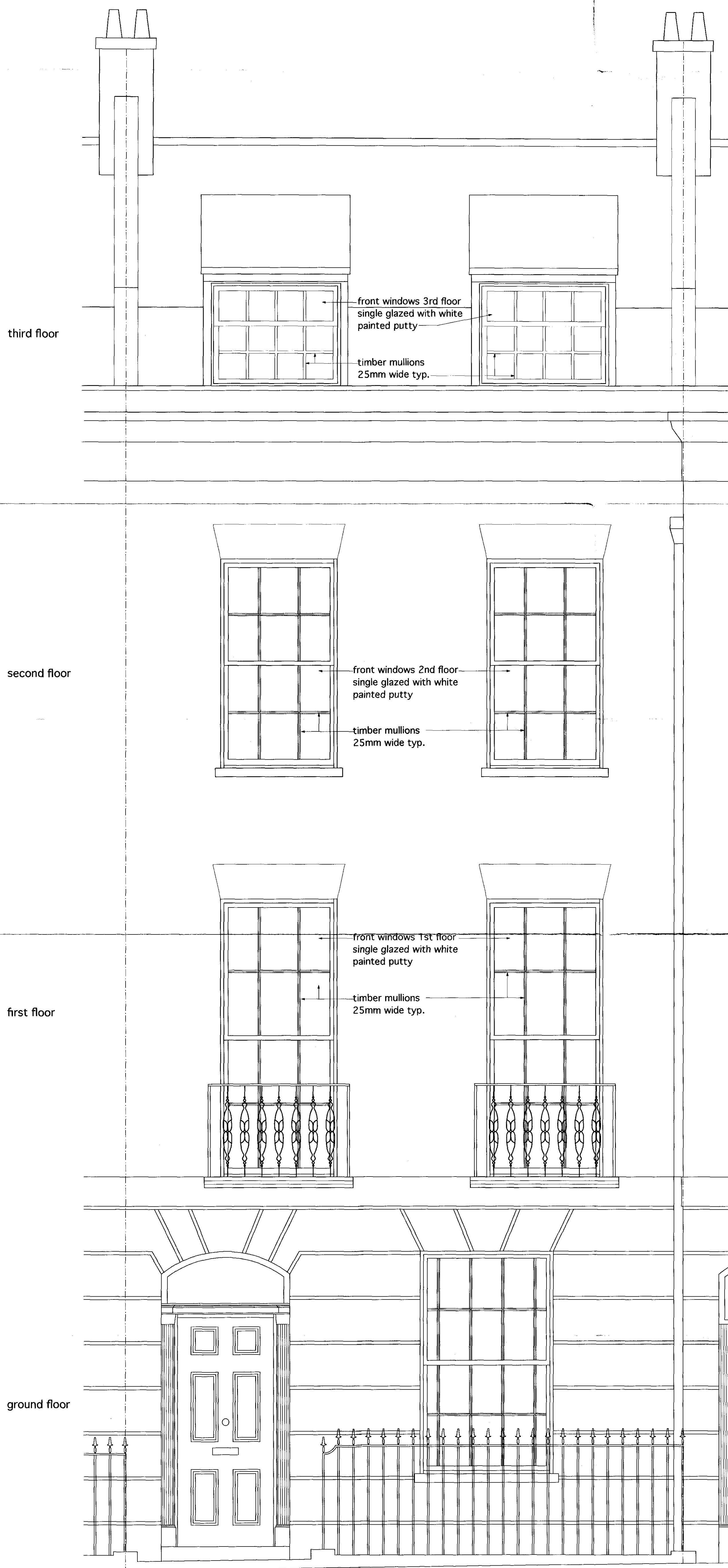
existing front elevation 1:20
