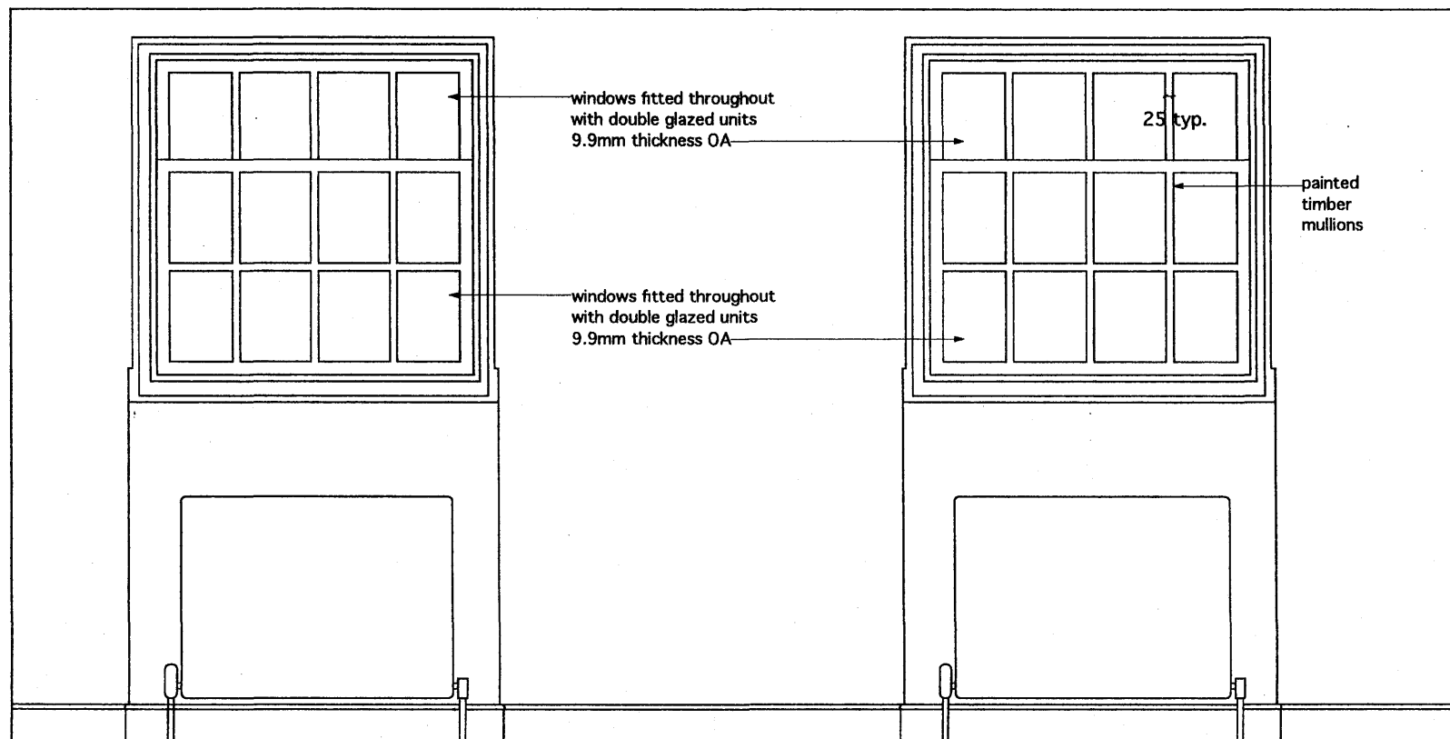
proposed internal elevation third floor front windows 1:20
