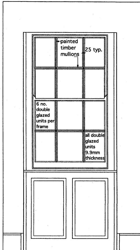
proposed internal elevation second floor rear stair window 1:20
