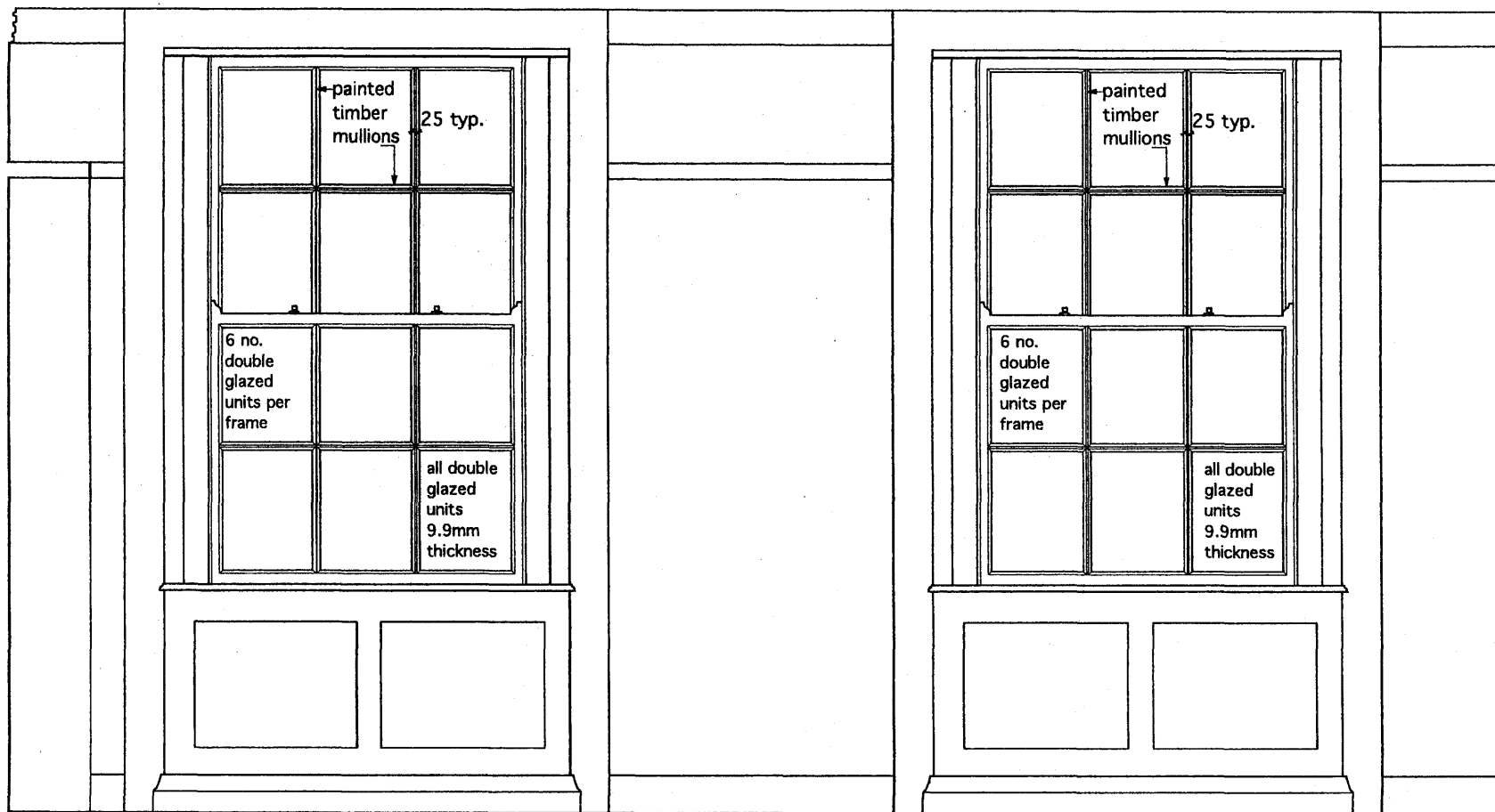
proposed internal elevation second floor front windows 1:20
