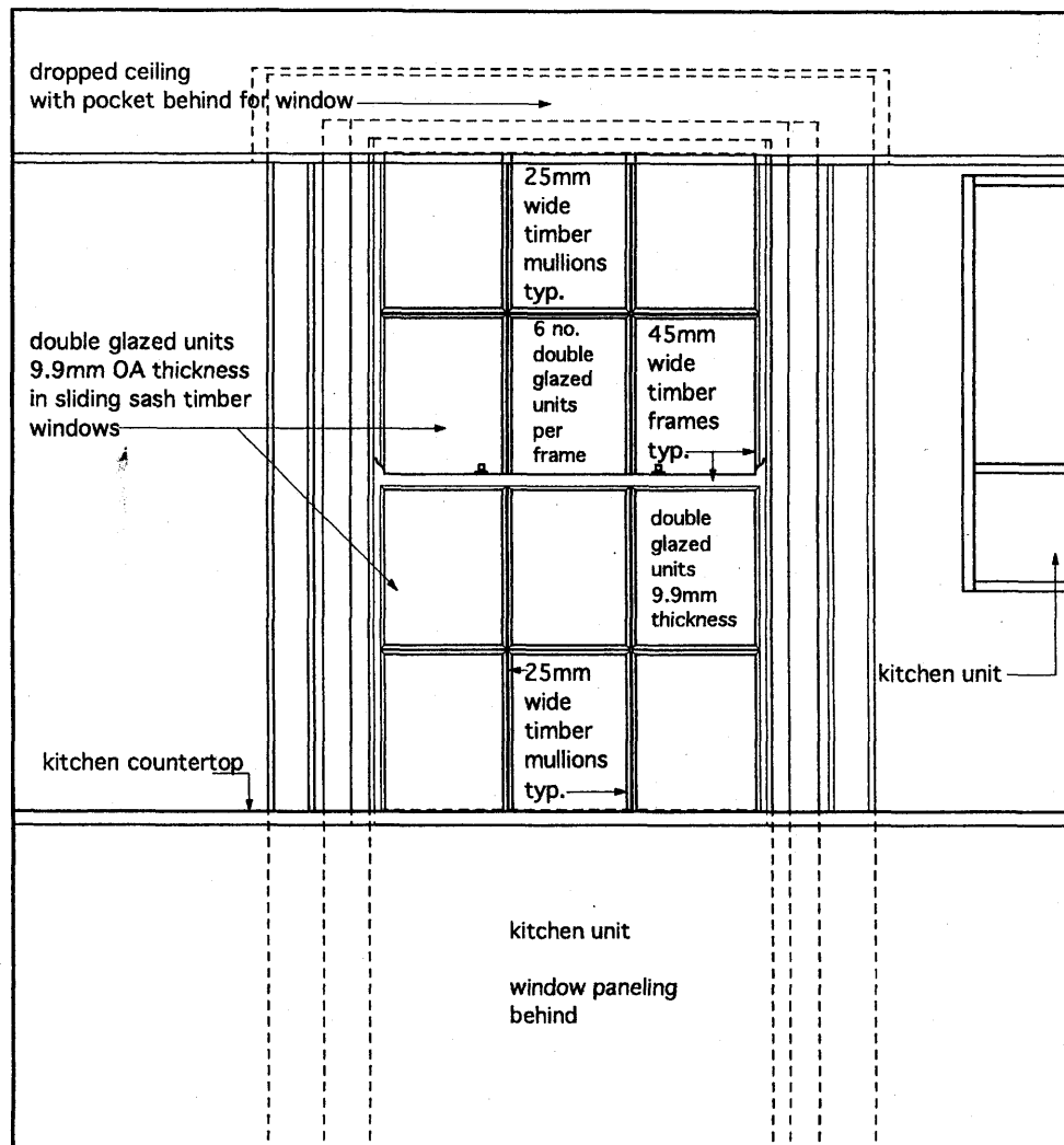
proposed internal elevation first floor rear window 1:20
