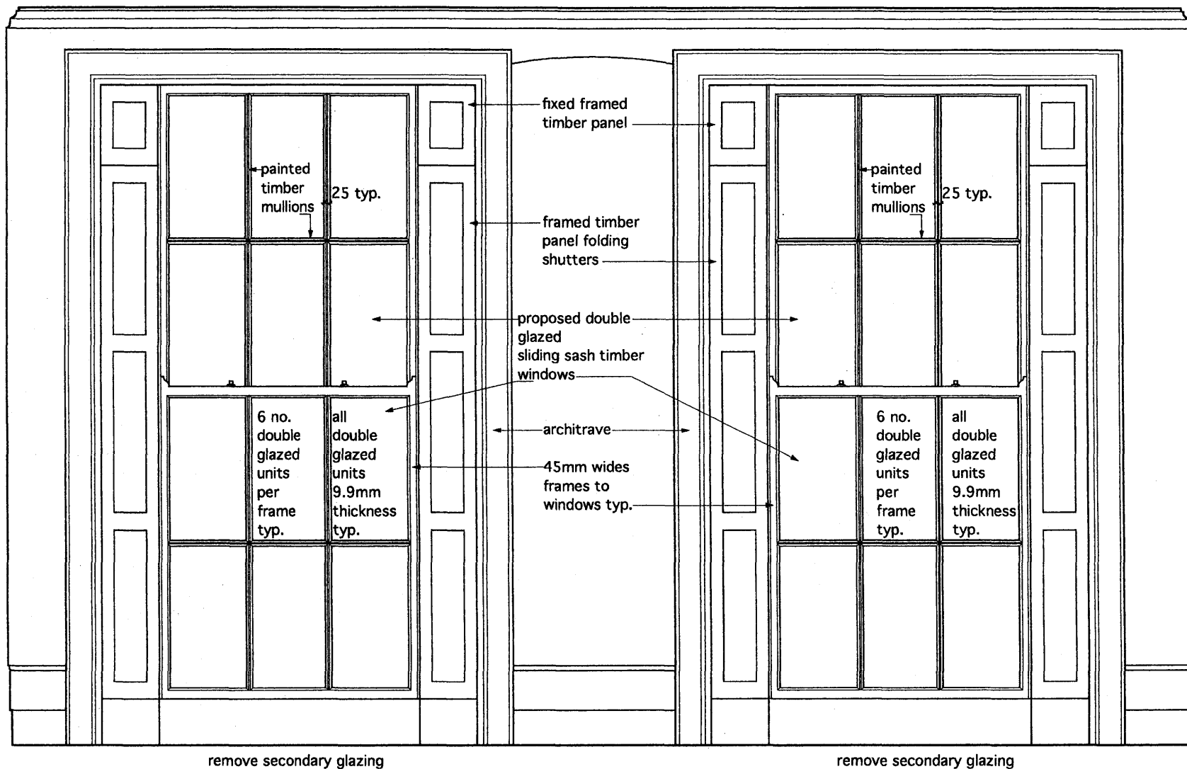
proposed elevation first floor front windows interior 1:20
