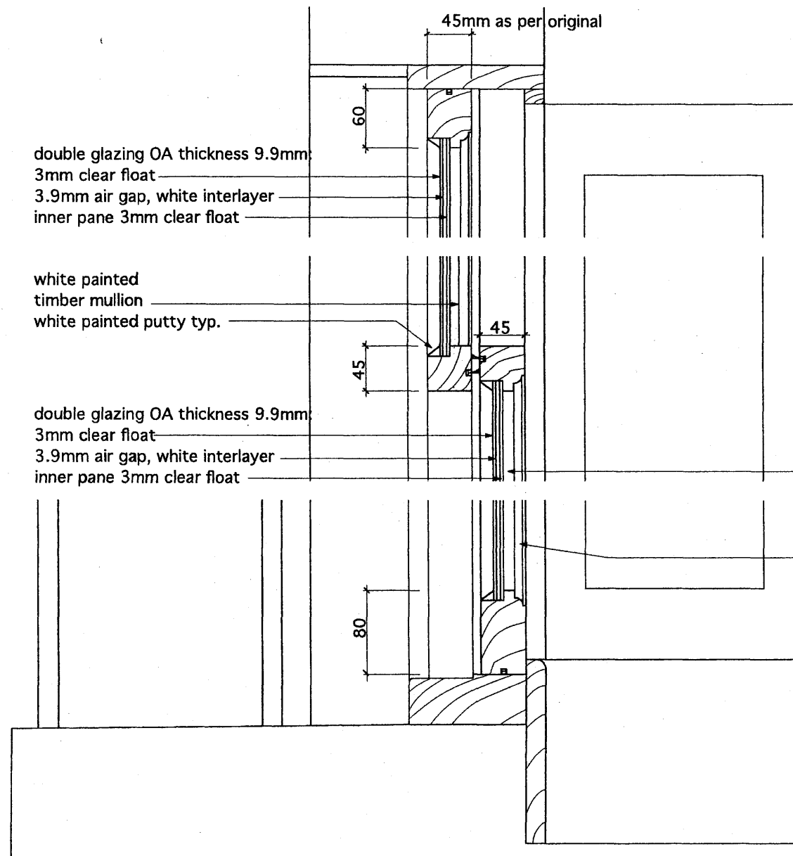
detail proposed vertical section first floor windows typ. 1:5
