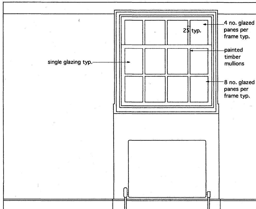
elevation existing third floor rear window interior 1:20
