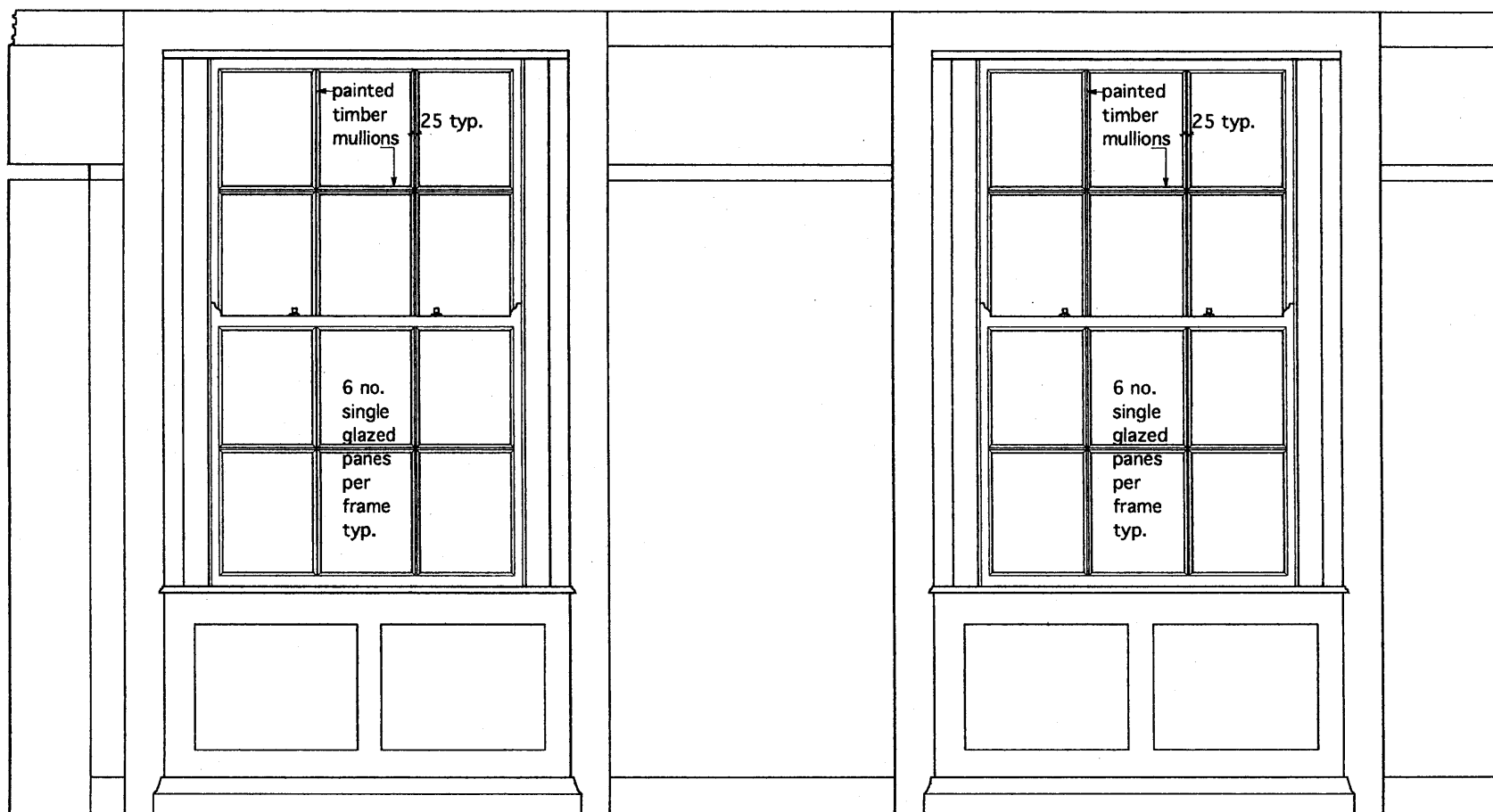
elevation existing second front windows interior 1:20
