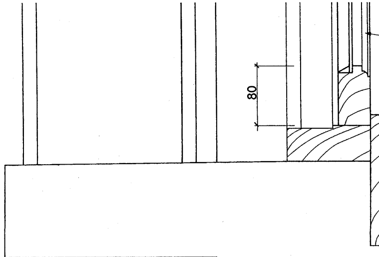
detail existing vertical section first floor windows typ. 1:5
