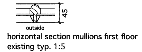
sliding sash single glazed timber windows
