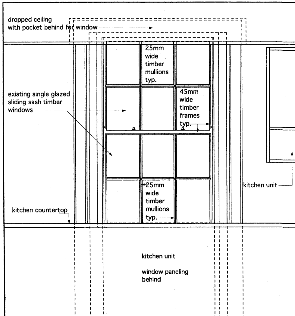
elevation existing first floor rear window interior 1:20
